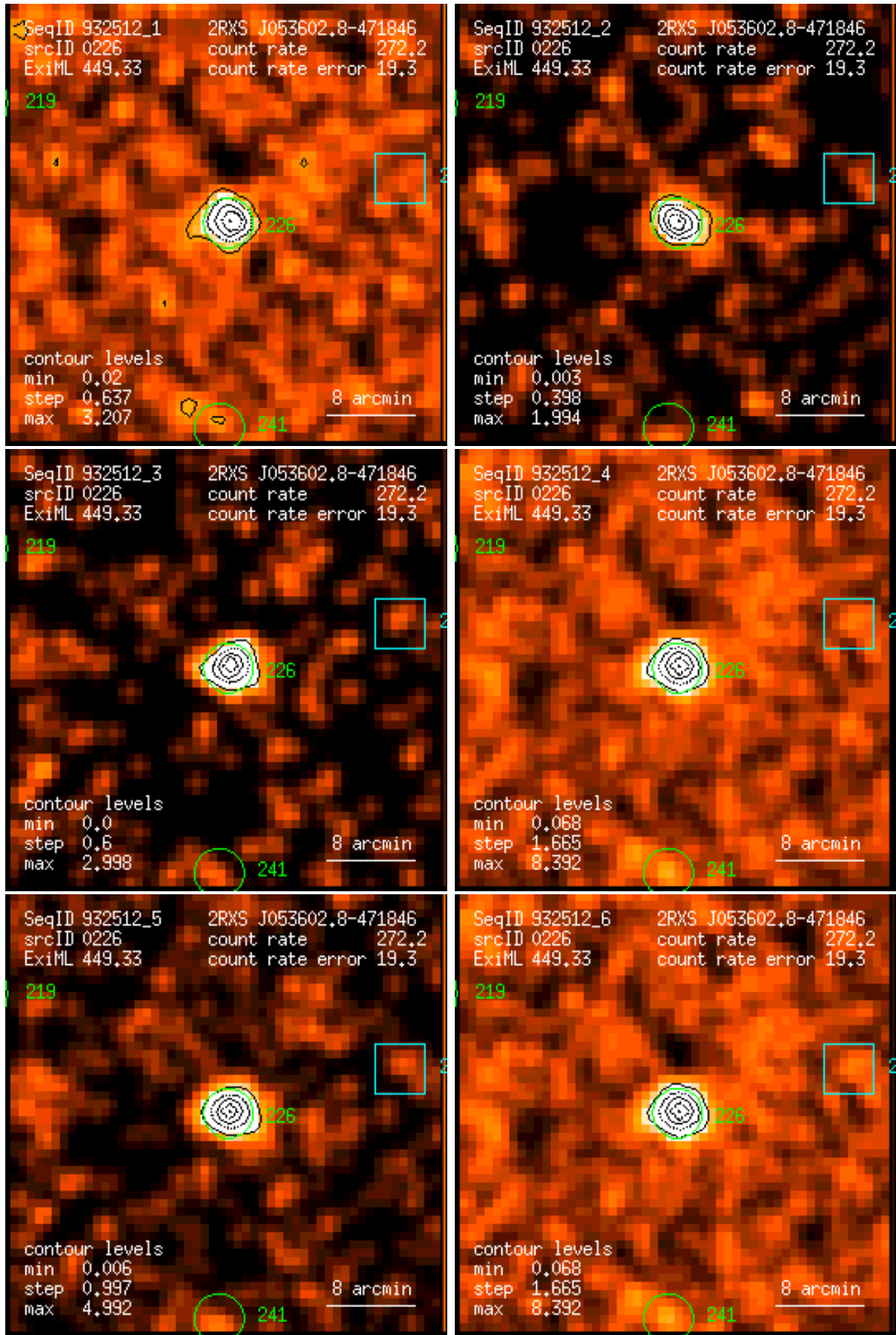
Figure 226: RASS 932512: detection 0226: band rate images, Gaussian filter: (1) PSPC channels 11 – 41, (2) 52 – 90, (3) 91 – 201, (4) 11 – 235, (5) 52 – 201, (6) 11 – 201. Broad band rates in counts/ks. Band rate contour levels in counts/ks/arcmin 2 .
