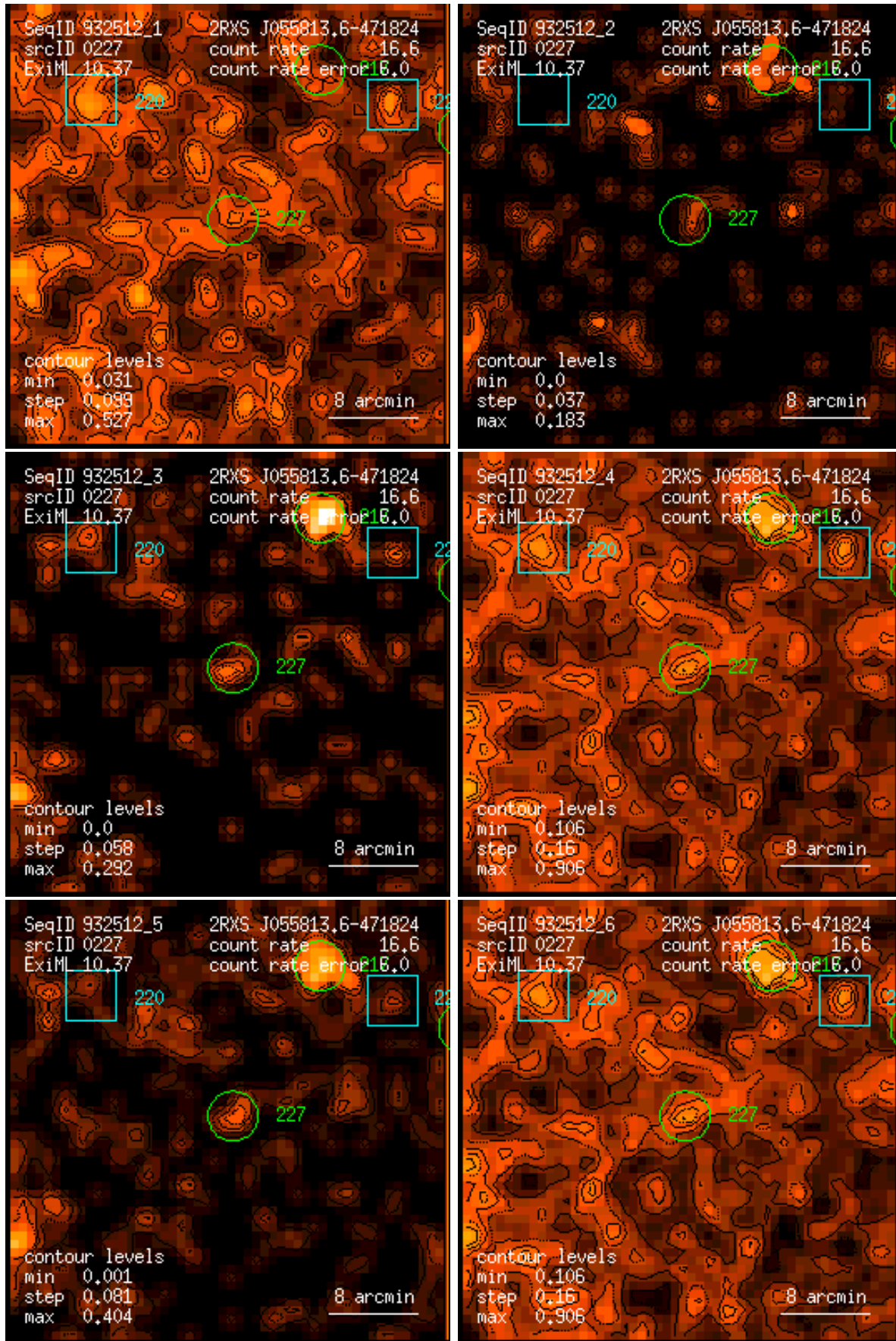
Figure 227: RASS 932512: detection 0227: band rate images, Gaussian filter: (1) PSPC channels 11 – 41, (2) 52 – 90, (3) 91 – 201, (4) 11 – 235, (5) 52 – 201, (6) 11 – 201. Broad band rates in counts/ks. Band rate contour levels in counts/ks/arcmin 2 .
