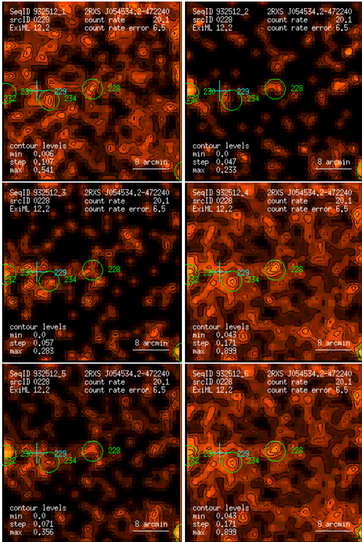
Figure 228: RASS 932512: detection 0228: band rate images, Gaussian filter: (1) PSPC channels 11 – 41, (2) 52 – 90, (3) 91 – 201, (4) 11 – 235, (5) 52 – 201, (6) 11 – 201. Broad band rates in counts/ks. Band rate contour levels in counts/ks/arcmin 2 .
