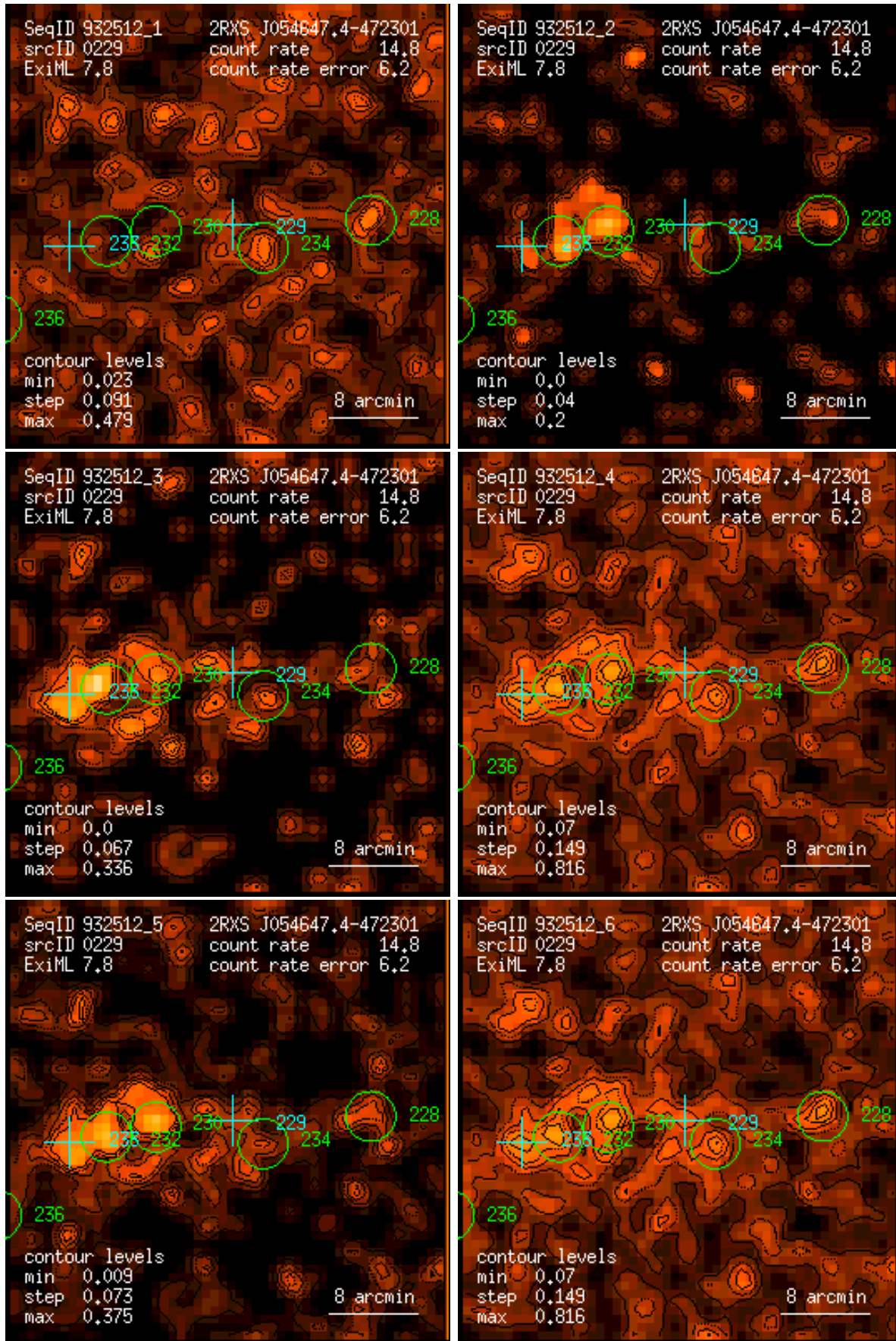
Figure 229: RASS 932512: detection 0229: band rate images, Gaussian filter: (1) PSPC channels 11 – 41, (2) 52 – 90, (3) 91 – 201, (4) 11 – 235, (5) 52 – 201, (6) 11 – 201. Broad band rates in counts/ks. Band rate contour levels in counts/ks/arcmin 2 .
