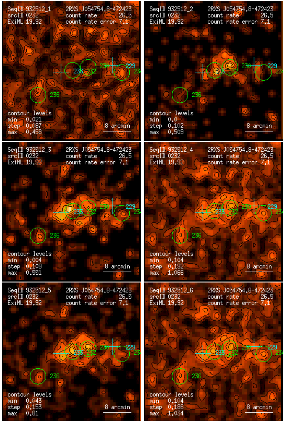
Figure 232: RASS 932512: detection 0232: band rate images, Gaussian filter: (1) PSPC channels 11 – 41, (2) 52 – 90, (3) 91 – 201, (4) 11 – 235, (5) 52 – 201, (6) 11 – 201. Broad band rates in counts/ks. Band rate contour levels in counts/ks/arcmin 2 .
