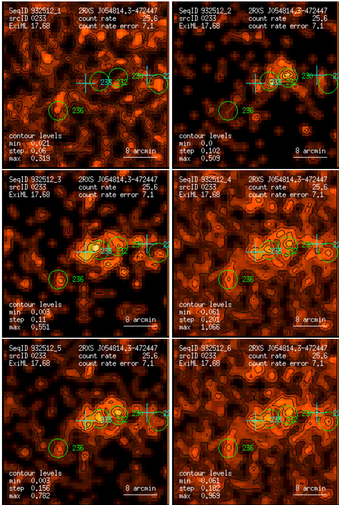
Figure 233: RASS 932512: detection 0233: band rate images, Gaussian filter: (1) PSPC channels 11 – 41, (2) 52 – 90, (3) 91 – 201, (4) 11 – 235, (5) 52 – 201, (6) 11 – 201. Broad band rates in counts/ks. Band rate contour levels in counts/ks/arcmin 2 .
