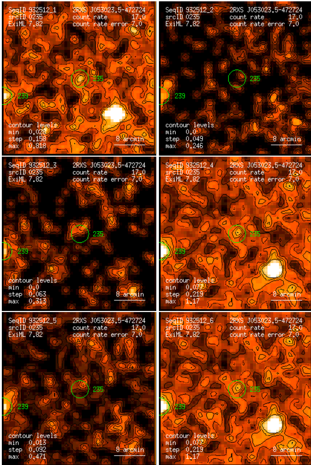
Figure 235: RASS 932512: detection 0235: band rate images, Gaussian filter: (1) PSPC channels 11 – 41, (2) 52 – 90, (3) 91 – 201, (4) 11 – 235, (5) 52 – 201, (6) 11 – 201. Broad band rates in counts/ks. Band rate contour levels in counts/ks/arcmin 2 .
