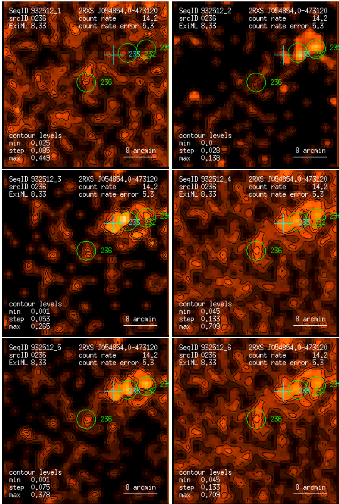
Figure 236: RASS 932512: detection 0236: band rate images, Gaussian filter: (1) PSPC channels 11 – 41, (2) 52 – 90, (3) 91 – 201, (4) 11 – 235, (5) 52 – 201, (6) 11 – 201. Broad band rates in counts/ks. Band rate contour levels in counts/ks/arcmin 2 .
