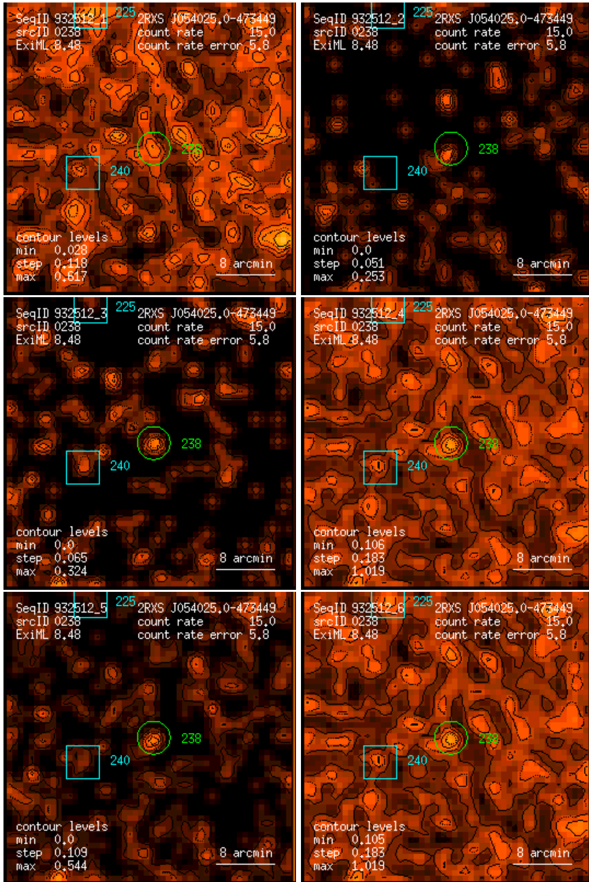
Figure 238: RASS 932512: detection 0238: band rate images, Gaussian filter: (1) PSPC channels 11 – 41, (2) 52 – 90, (3) 91 – 201, (4) 11 – 235, (5) 52 – 201, (6) 11 – 201. Broad band rates in counts/ks. Band rate contour levels in counts/ks/arcmin 2 .
