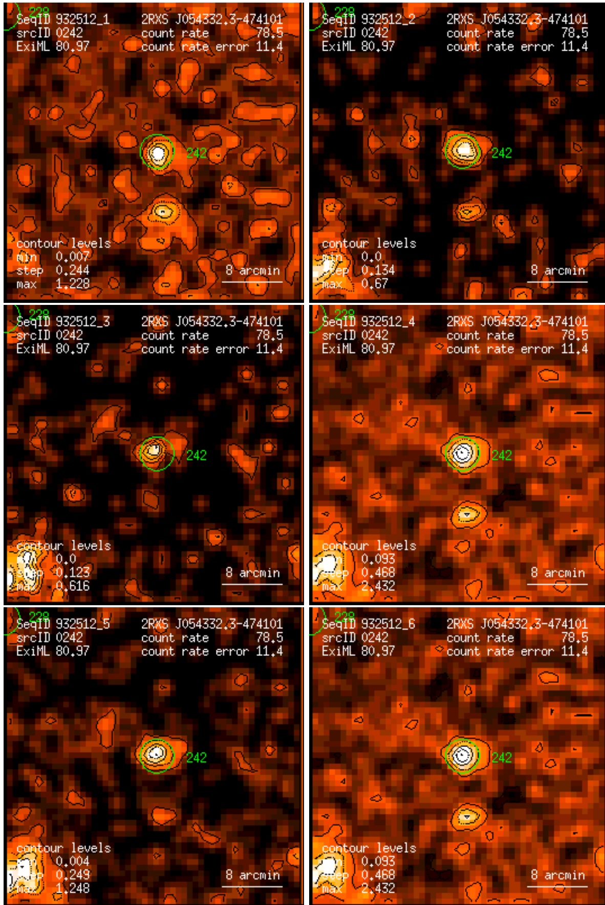
Figure 242: RASS 932512: detection 0242: band rate images, Gaussian filter: (1) PSPC channels 11 – 41, (2) 52 – 90, (3) 91 – 201, (4) 11 – 235, (5) 52 – 201, (6) 11 – 201. Broad band rates in counts/ks. Band rate contour levels in counts/ks/arcmin 2 .
