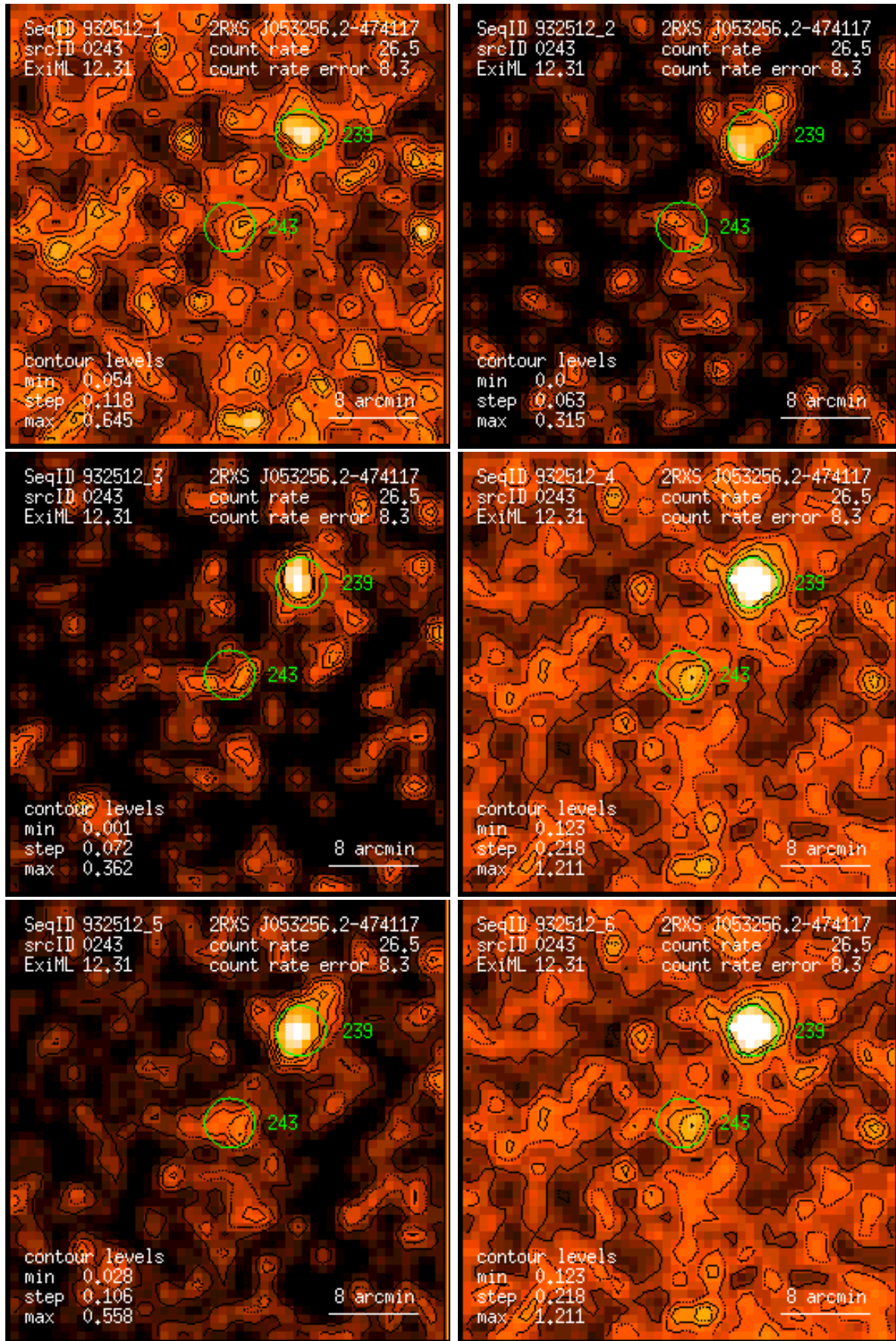
Figure 243: RASS 932512: detection 0243: band rate images, Gaussian filter: (1) PSPC channels 11 – 41, (2) 52 – 90, (3) 91 – 201, (4) 11 – 235, (5) 52 – 201, (6) 11 – 201. Broad band rates in counts/ks. Band rate contour levels in counts/ks/arcmin 2 .
