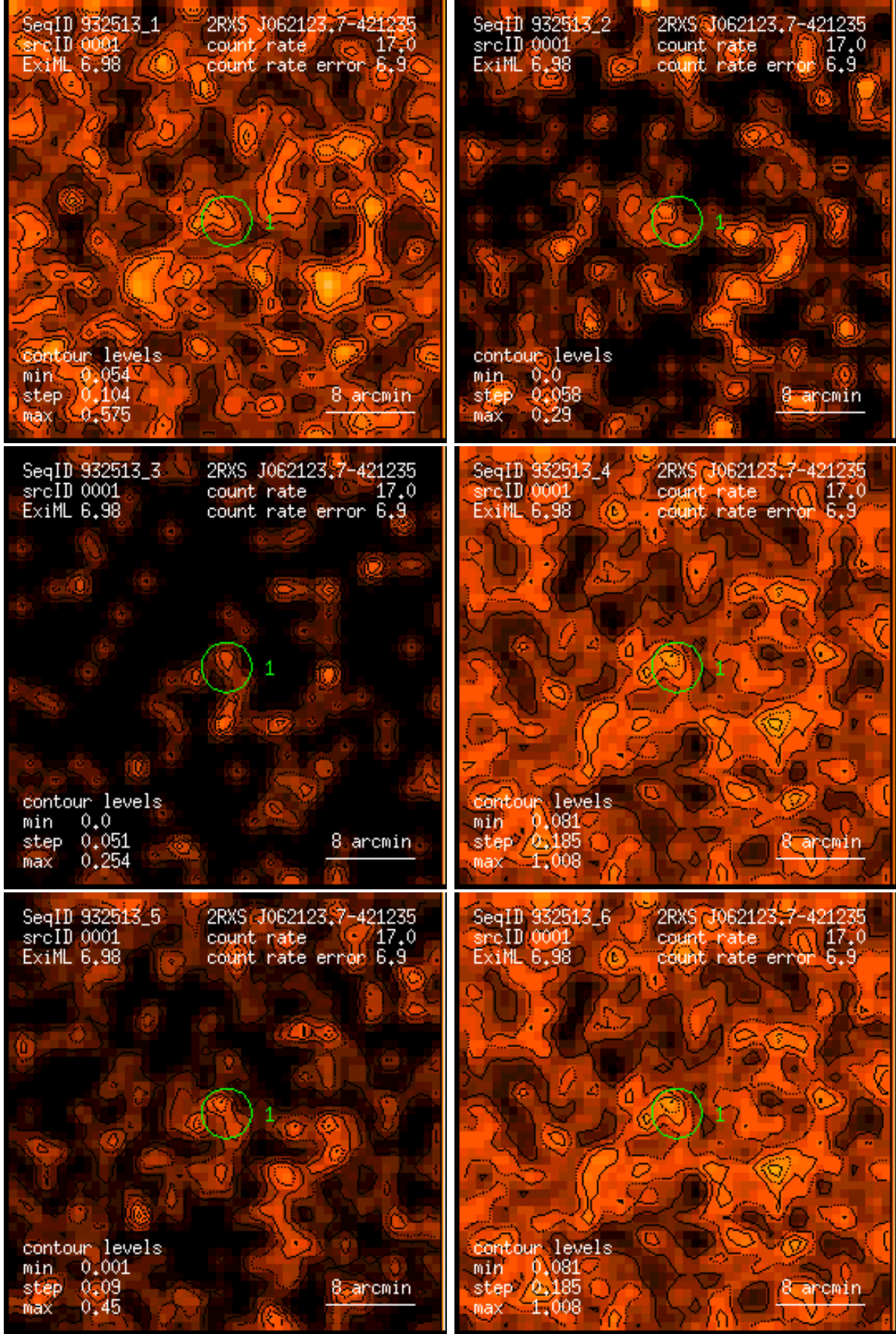
Figure 1: RASS 932513: detection 0001: band rate images, Gaussian filter: (1) PSPC channels 11 – 41, (2) 52 – 90, (3) 91 – 201, (4) 11 – 235, (5) 52 – 201, (6) 11 – 201. Broad band rates in counts/ks. Band rate contour levels in counts/ks/arcmin 2 .
