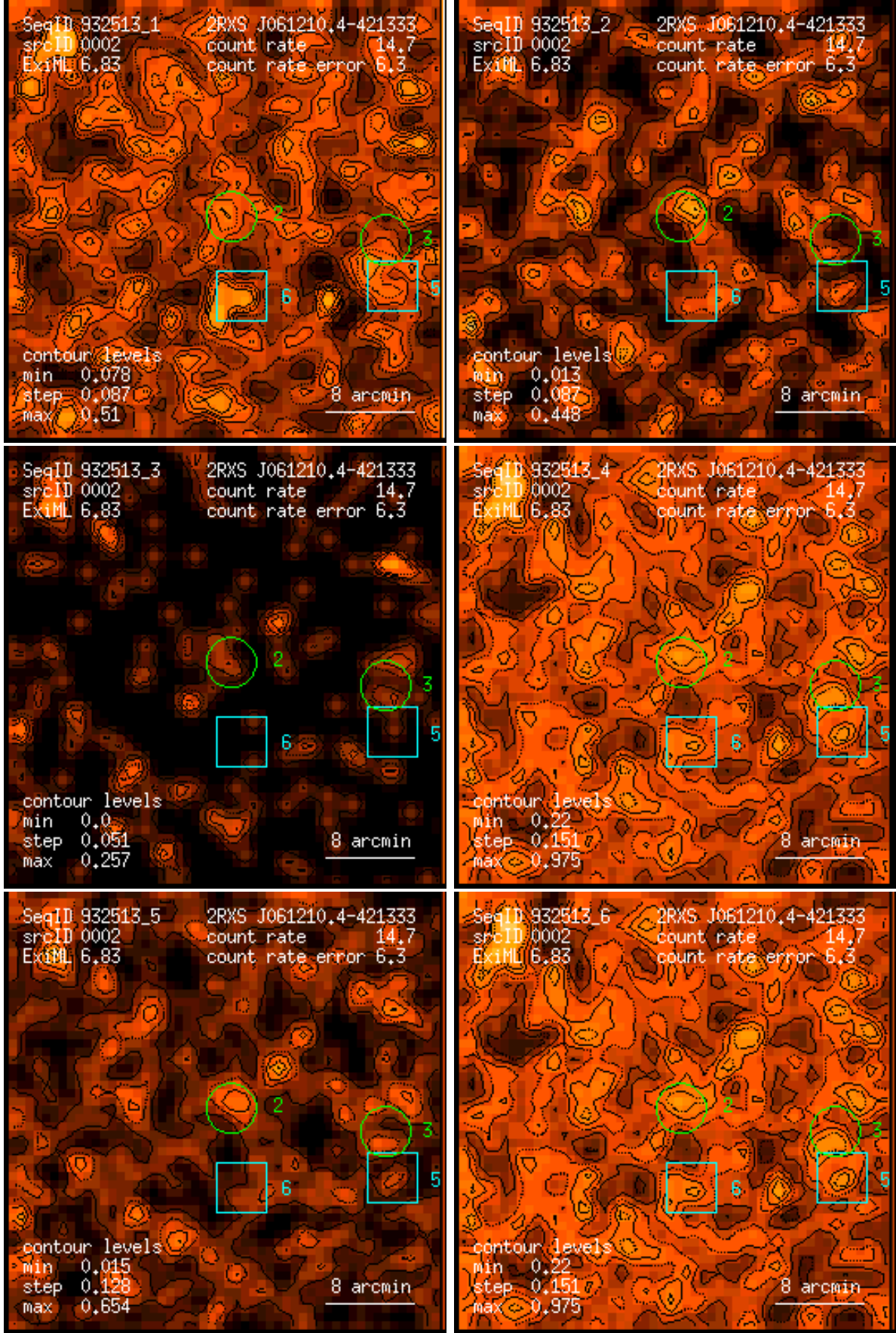
Figure 2: RASS 932513: detection 0002: band rate images, Gaussian filter: (1) PSPC channels 11 – 41, (2) 52 – 90, (3) 91 – 201, (4) 11 – 235, (5) 52 – 201, (6) 11 – 201. Broad band rates in counts/ks. Band rate contour levels in counts/ks/arcmin 2 .
