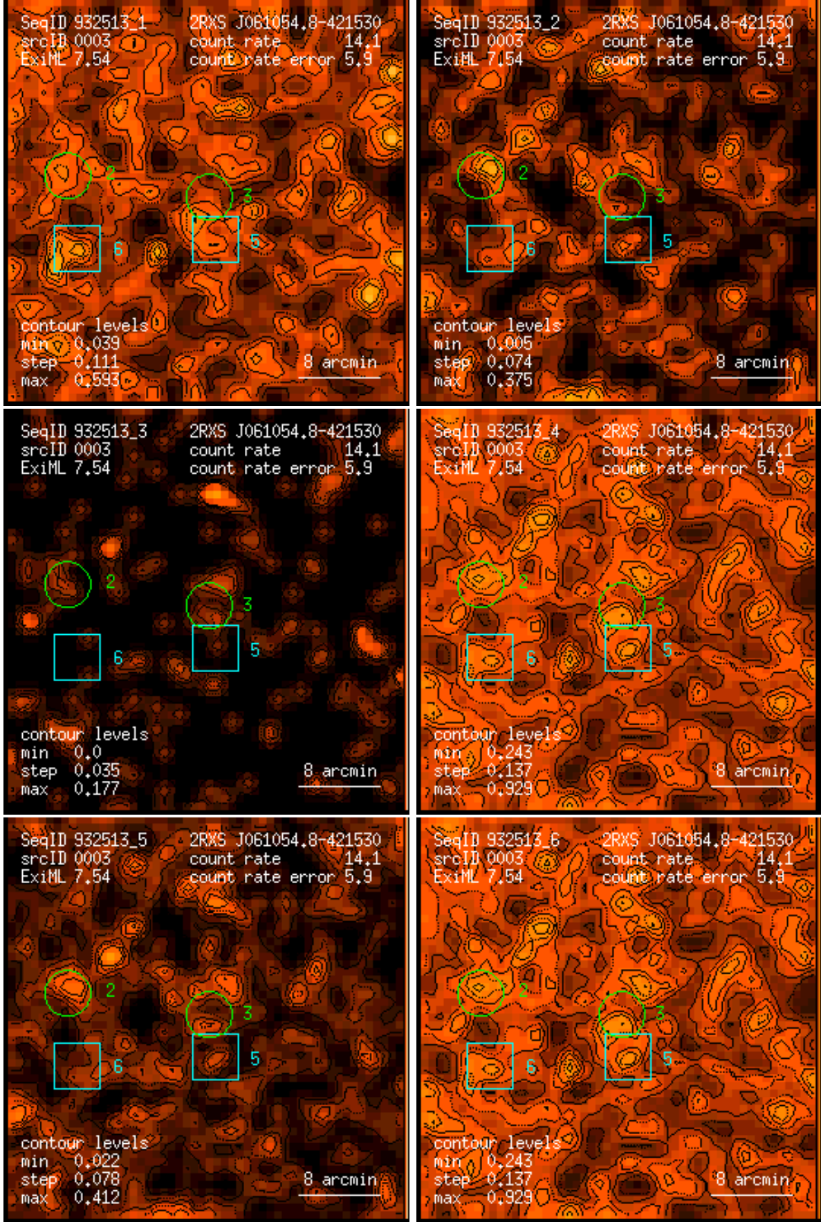
Figure 3: RASS 932513: detection 0003: band rate images, Gaussian filter: (1) PSPC channels 11 – 41, (2) 52 – 90, (3) 91 – 201, (4) 11 – 235, (5) 52 – 201, (6) 11 – 201. Broad band rates in counts/ks. Band rate contour levels in counts/ks/arcmin 2 .
