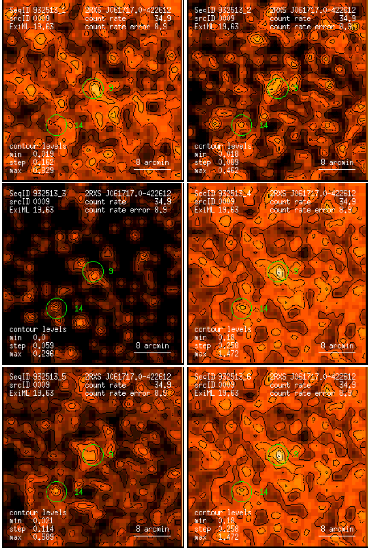
Figure 9: RASS 932513: detection 0009: band rate images, Gaussian filter: (1) PSPC channels 11 – 41, (2) 52 – 90, (3) 91 – 201, (4) 11 – 235, (5) 52 – 201, (6) 11 – 201. Broad band rates in counts/ks. Band rate contour levels in counts/ks/arcmin 2 .
