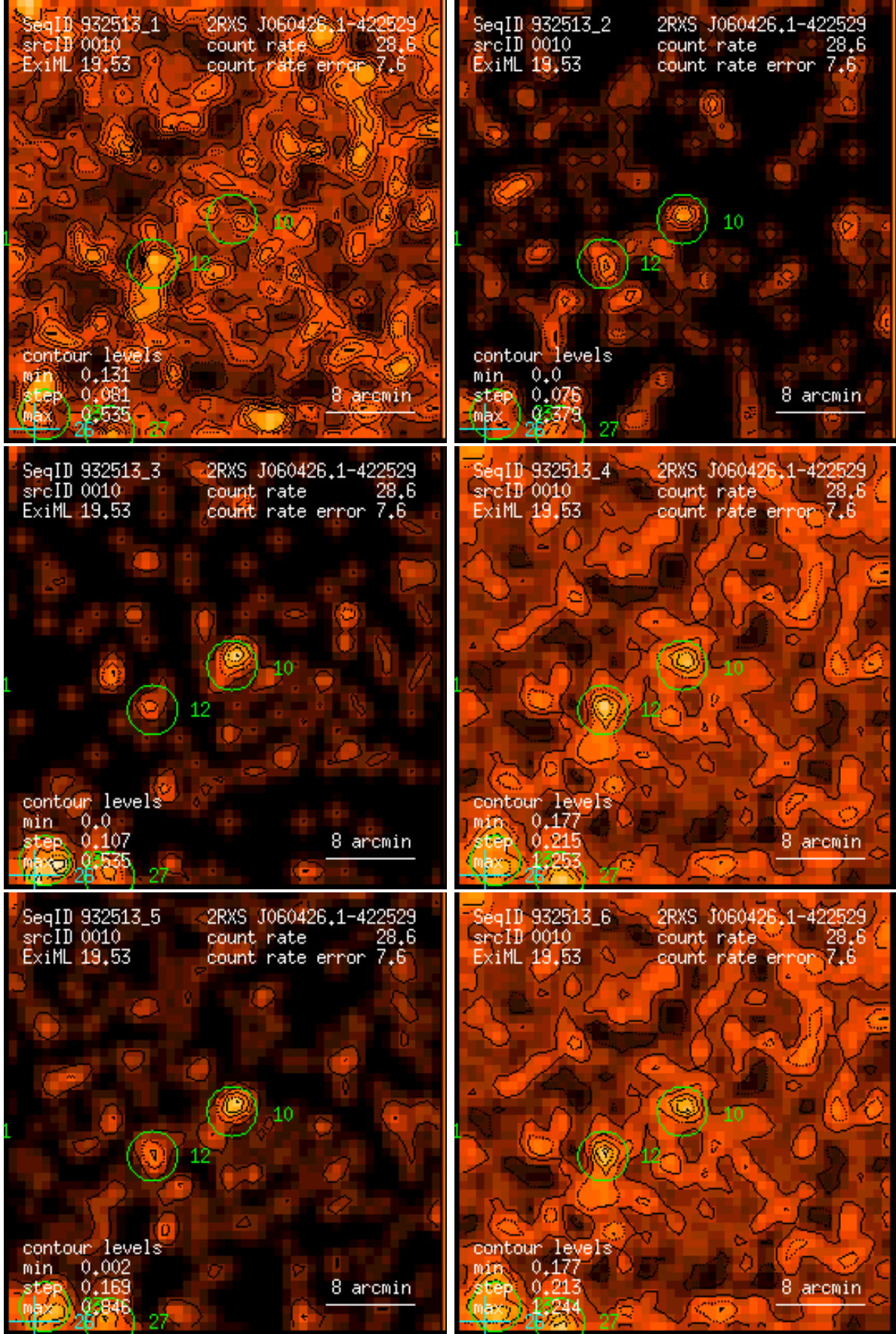
Figure 10: RASS 932513: detection 0010: band rate images, Gaussian filter: (1) PSPC channels 11 – 41, (2) 52 – 90, (3) 91 – 201, (4) 11 – 235, (5) 52 – 201, (6) 11 – 201. Broad band rates in counts/ks. Band rate contour levels in counts/ks/arcmin 2 .
