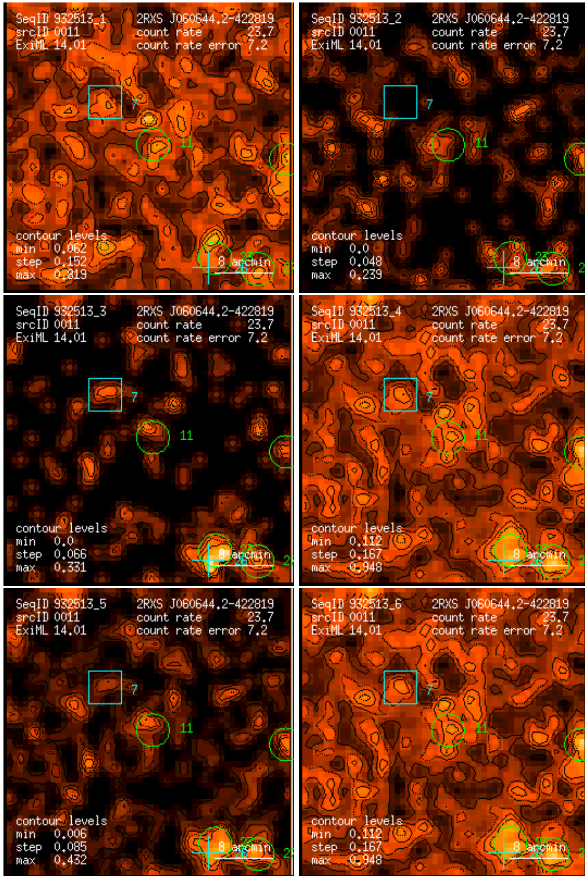
Figure 11: RASS 932513: detection 0011: band rate images, Gaussian filter: (1) PSPC channels 11 – 41, (2) 52 – 90, (3) 91 – 201, (4) 11 – 235, (5) 52 – 201, (6) 11 – 201. Broad band rates in counts/ks. Band rate contour levels in counts/ks/arcmin 2 .
