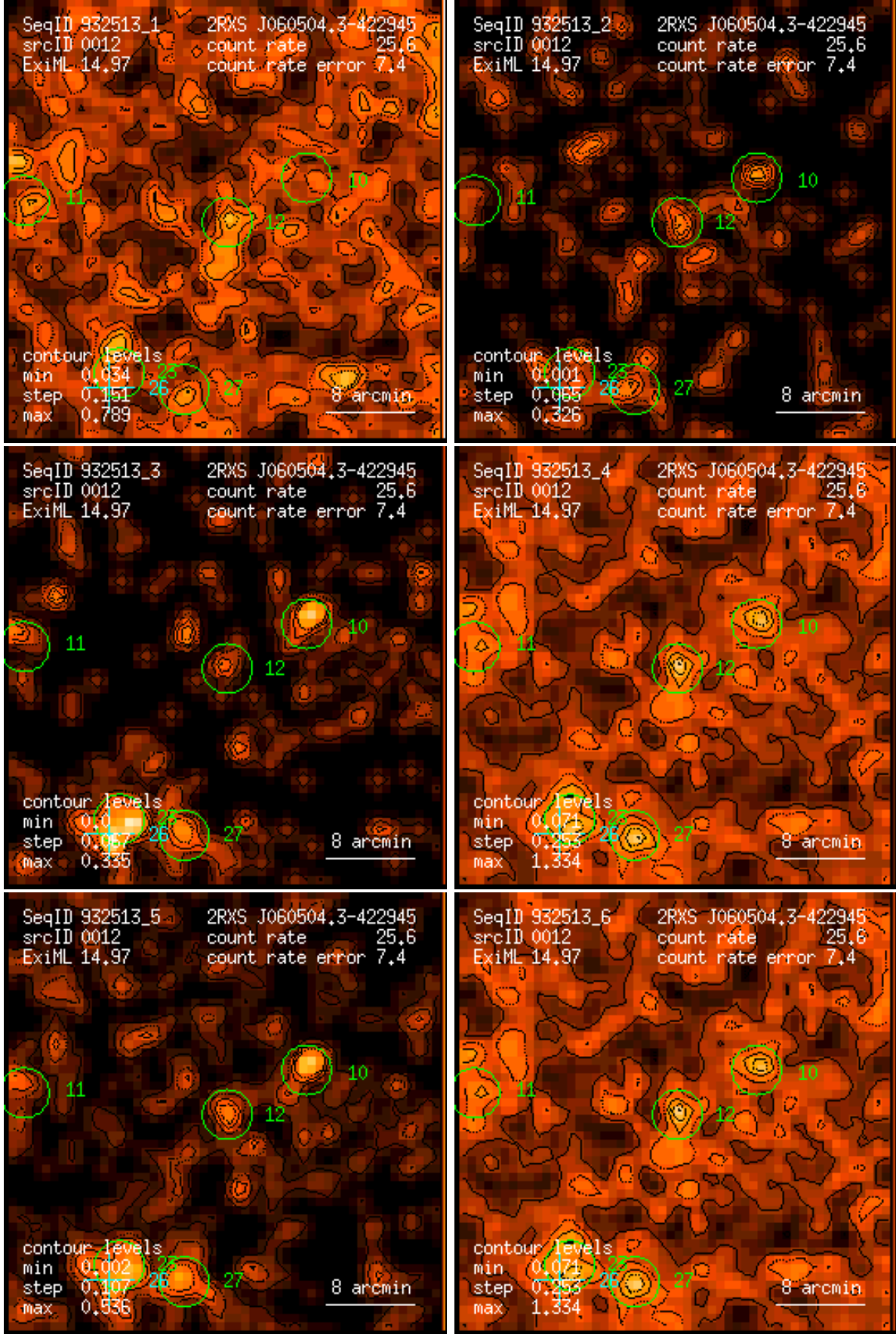
Figure 12: RASS 932513: detection 0012: band rate images, Gaussian filter: (1) PSPC channels 11 – 41, (2) 52 – 90, (3) 91 – 201, (4) 11 – 235, (5) 52 – 201, (6) 11 – 201. Broad band rates in counts/ks. Band rate contour levels in counts/ks/arcmin 2 .
