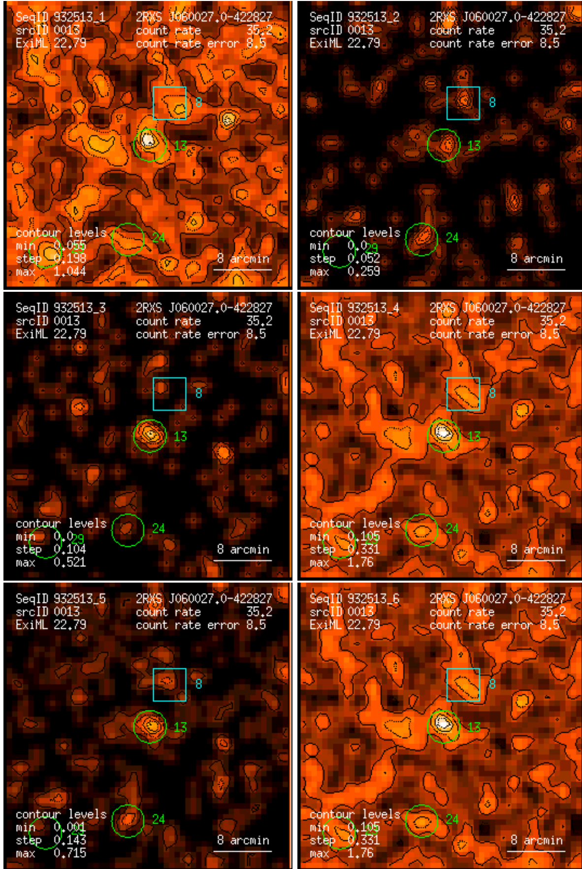
Figure 13: RASS 932513: detection 0013: band rate images, Gaussian filter: (1) PSPC channels 11 – 41, (2) 52 – 90, (3) 91 – 201, (4) 11 – 235, (5) 52 – 201, (6) 11 – 201. Broad band rates in counts/ks. Band rate contour levels in counts/ks/arcmin 2 .
