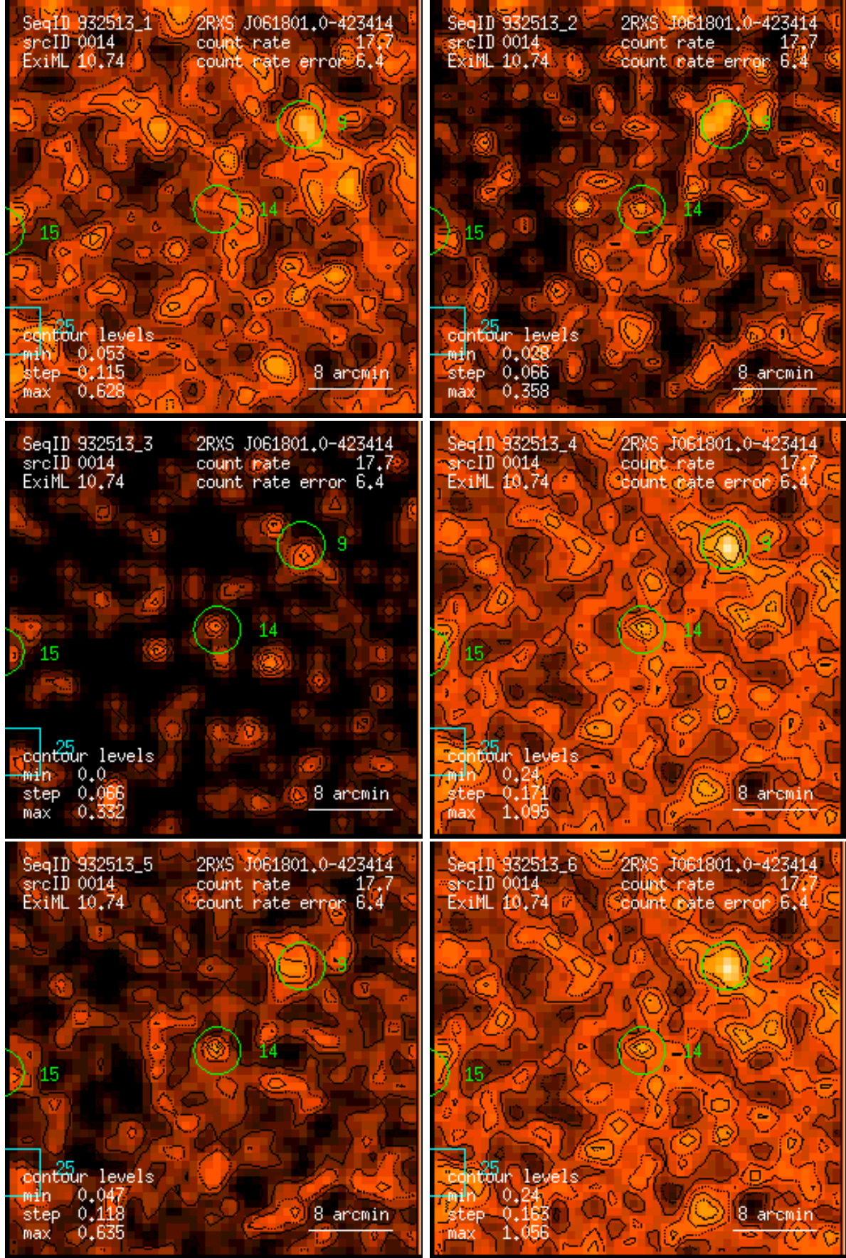
Figure 14: RASS 932513: detection 0014: band rate images, Gaussian filter: (1) PSPC channels 11 – 41, (2) 52 – 90, (3) 91 – 201, (4) 11 – 235, (5) 52 – 201, (6) 11 – 201. Broad band rates in counts/ks. Band rate contour levels in counts/ks/arcmin 2 .
