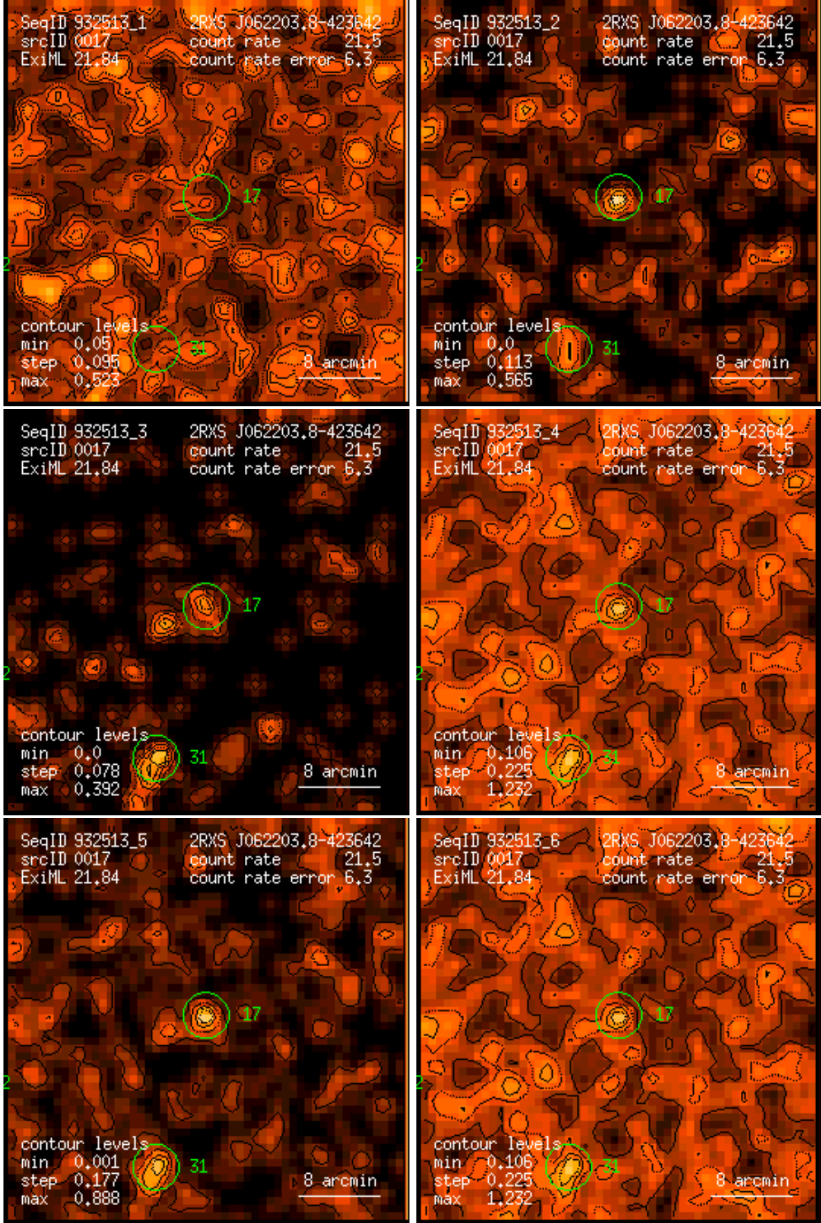
Figure 17: RASS 932513: detection 0017: band rate images, Gaussian filter: (1) PSPC channels 11 – 41, (2) 52 – 90, (3) 91 – 201, (4) 11 – 235, (5) 52 – 201, (6) 11 – 201. Broad band rates in counts/ks. Band rate contour levels in counts/ks/arcmin 2 .
