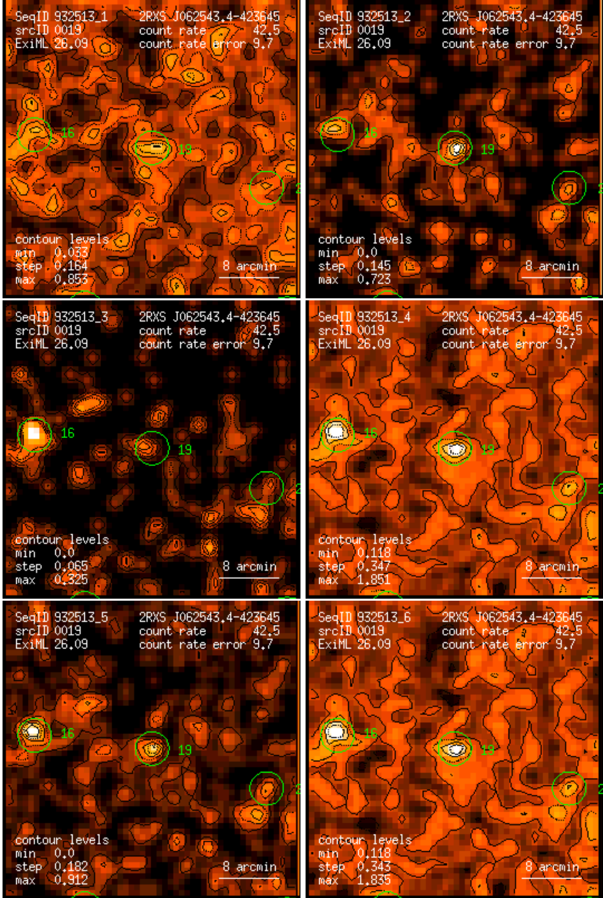
Figure 19: RASS 932513: detection 0019: band rate images, Gaussian filter: (1) PSPC channels 11 – 41, (2) 52 – 90, (3) 91 – 201, (4) 11 – 235, (5) 52 – 201, (6) 11 – 201. Broad band rates in counts/ks. Band rate contour levels in counts/ks/arcmin 2 .
