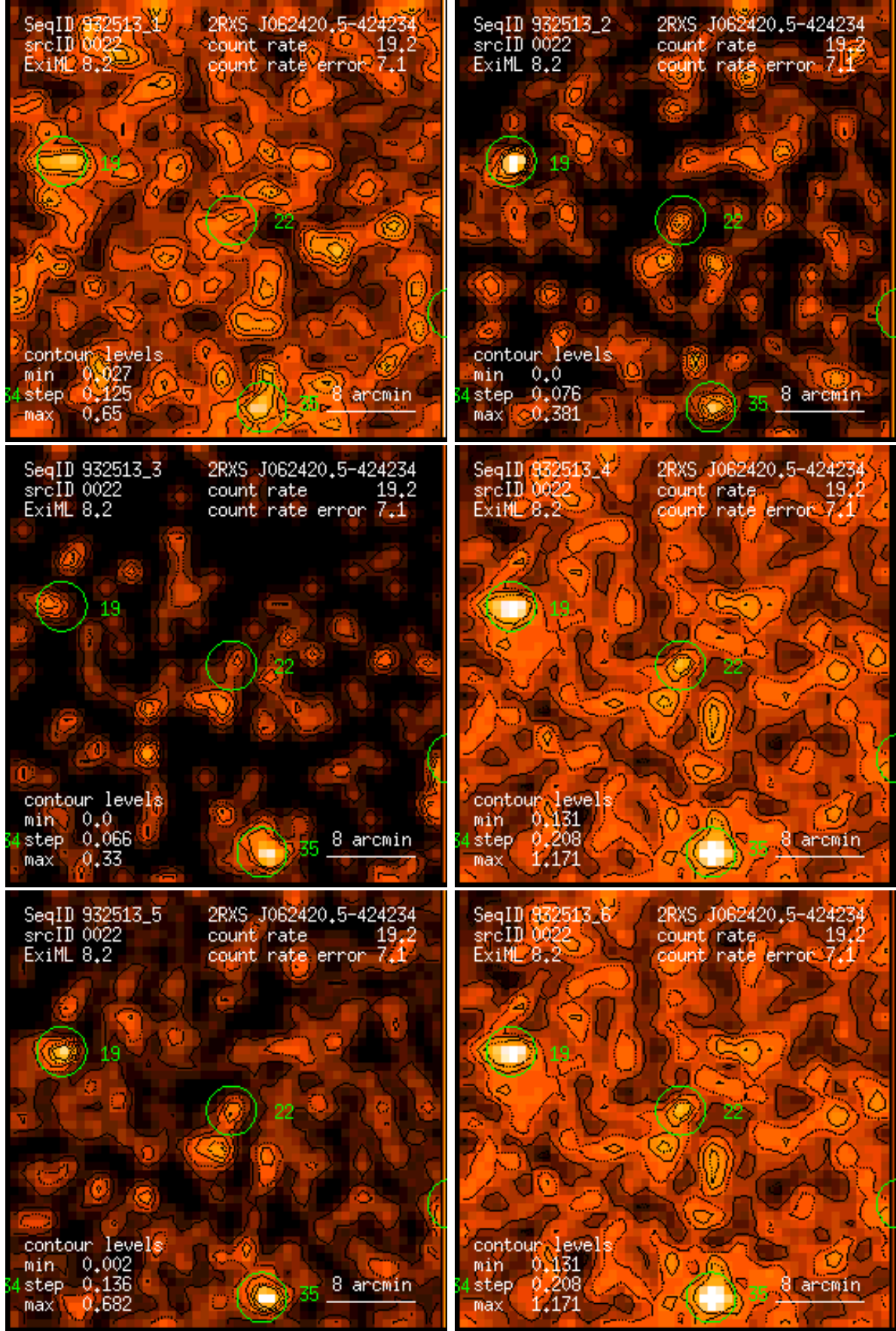
Figure 22: RASS 932513: detection 0022: band rate images, Gaussian filter: (1) PSPC channels 11 – 41, (2) 52 – 90, (3) 91 – 201, (4) 11 – 235, (5) 52 – 201, (6) 11 – 201. Broad band rates in counts/ks. Band rate contour levels in counts/ks/arcmin 2 .
