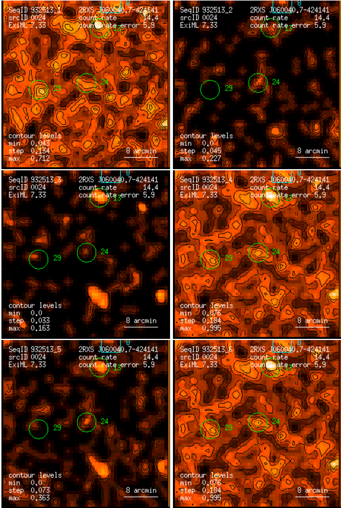
Figure 24: RASS 932513: detection 0024: band rate images, Gaussian filter: (1) PSPC channels 11 – 41, (2) 52 – 90, (3) 91 – 201, (4) 11 – 235, (5) 52 – 201, (6) 11 – 201. Broad band rates in counts/ks. Band rate contour levels in counts/ks/arcmin 2 .
