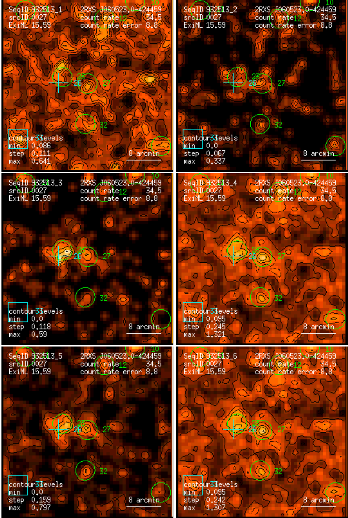
Figure 27: RASS 932513: detection 0027: band rate images, Gaussian filter: (1) PSPC channels 11 – 41, (2) 52 – 90, (3) 91 – 201, (4) 11 – 235, (5) 52 – 201, (6) 11 – 201. Broad band rates in counts/ks. Band rate contour levels in counts/ks/arcmin 2 .
