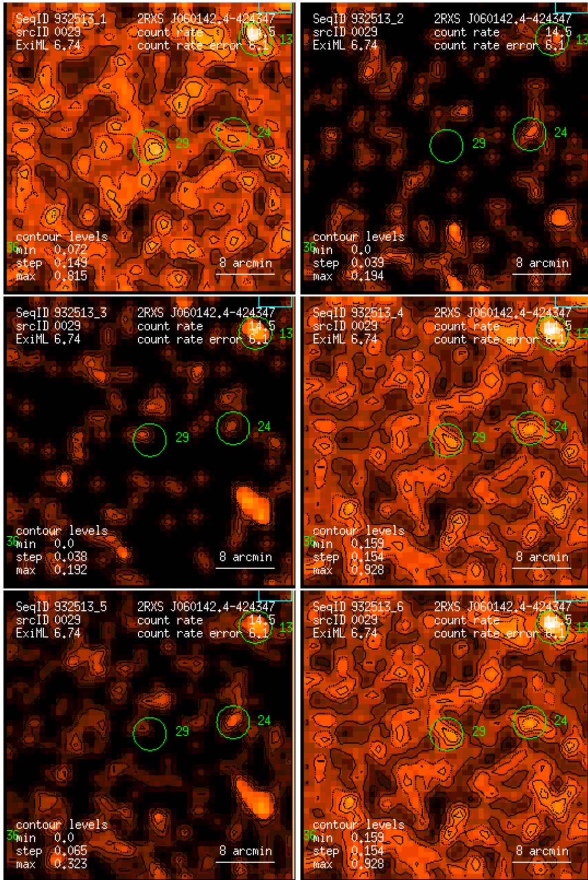
Figure 29: RASS 932513: detection 0029: band rate images, Gaussian filter: (1) PSPC channels 11 – 41, (2) 52 – 90, (3) 91 – 201, (4) 11 – 235, (5) 52 – 201, (6) 11 – 201. Broad band rates in counts/ks. Band rate contour levels in counts/ks/arcmin 2 .
