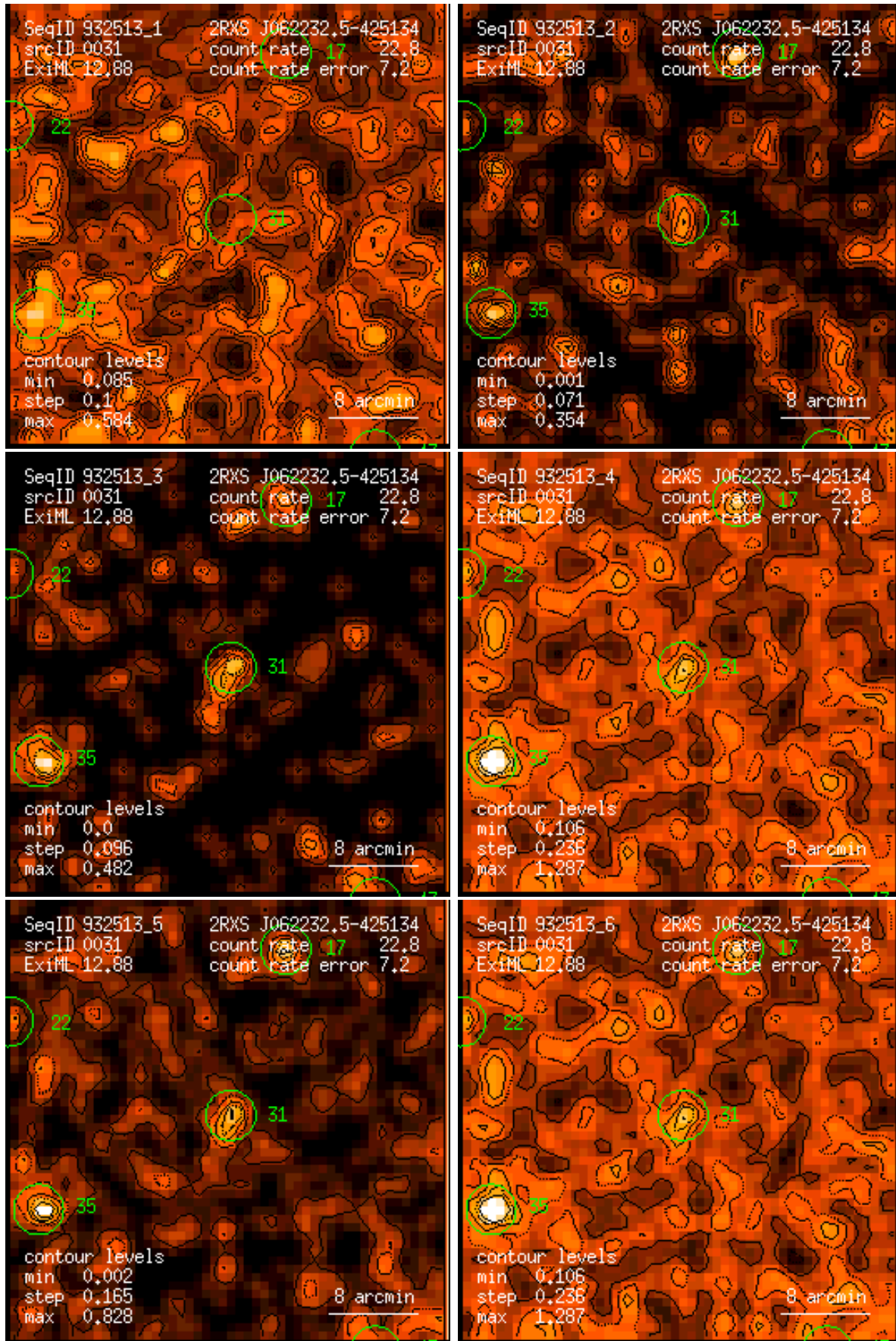
Figure 31: RASS 932513: detection 0031: band rate images, Gaussian filter: (1) PSPC channels 11 – 41, (2) 52 – 90, (3) 91 – 201, (4) 11 – 235, (5) 52 – 201, (6) 11 – 201. Broad band rates in counts/ks. Band rate contour levels in counts/ks/arcmin 2 .
