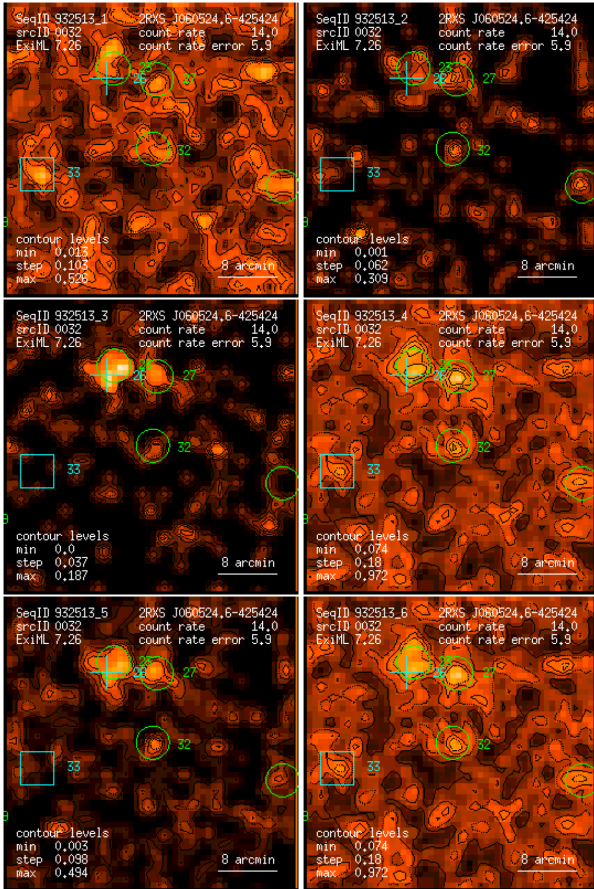
Figure 32: RASS 932513: detection 0032: band rate images, Gaussian filter: (1) PSPC channels 11 – 41, (2) 52 – 90, (3) 91 – 201, (4) 11 – 235, (5) 52 – 201, (6) 11 – 201. Broad band rates in counts/ks. Band rate contour levels in counts/ks/arcmin 2 .
