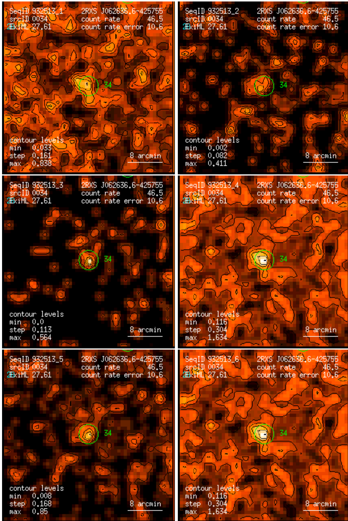
Figure 34: RASS 932513: detection 0034: band rate images, Gaussian filter: (1) PSPC channels 11 – 41, (2) 52 – 90, (3) 91 – 201, (4) 11 – 235, (5) 52 – 201, (6) 11 – 201. Broad band rates in counts/ks. Band rate contour levels in counts/ks/arcmin 2 .
