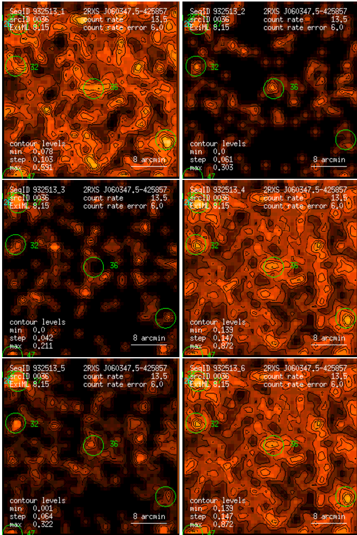
Figure 36: RASS 932513: detection 0036: band rate images, Gaussian filter: (1) PSPC channels 11 – 41, (2) 52 – 90, (3) 91 – 201, (4) 11 – 235, (5) 52 – 201, (6) 11 – 201. Broad band rates in counts/ks. Band rate contour levels in counts/ks/arcmin 2 .
