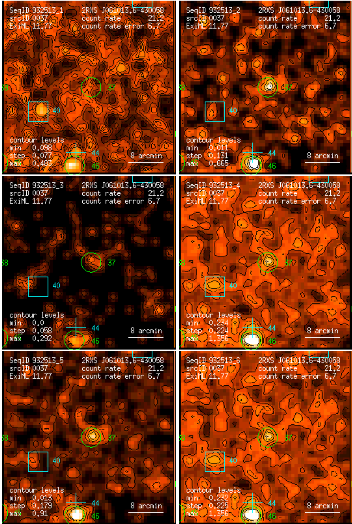
Figure 37: RASS 932513: detection 0037: band rate images, Gaussian filter: (1) PSPC channels 11 – 41, (2) 52 – 90, (3) 91 – 201, (4) 11 – 235, (5) 52 – 201, (6) 11 – 201. Broad band rates in counts/ks. Band rate contour levels in counts/ks/arcmin 2 .
