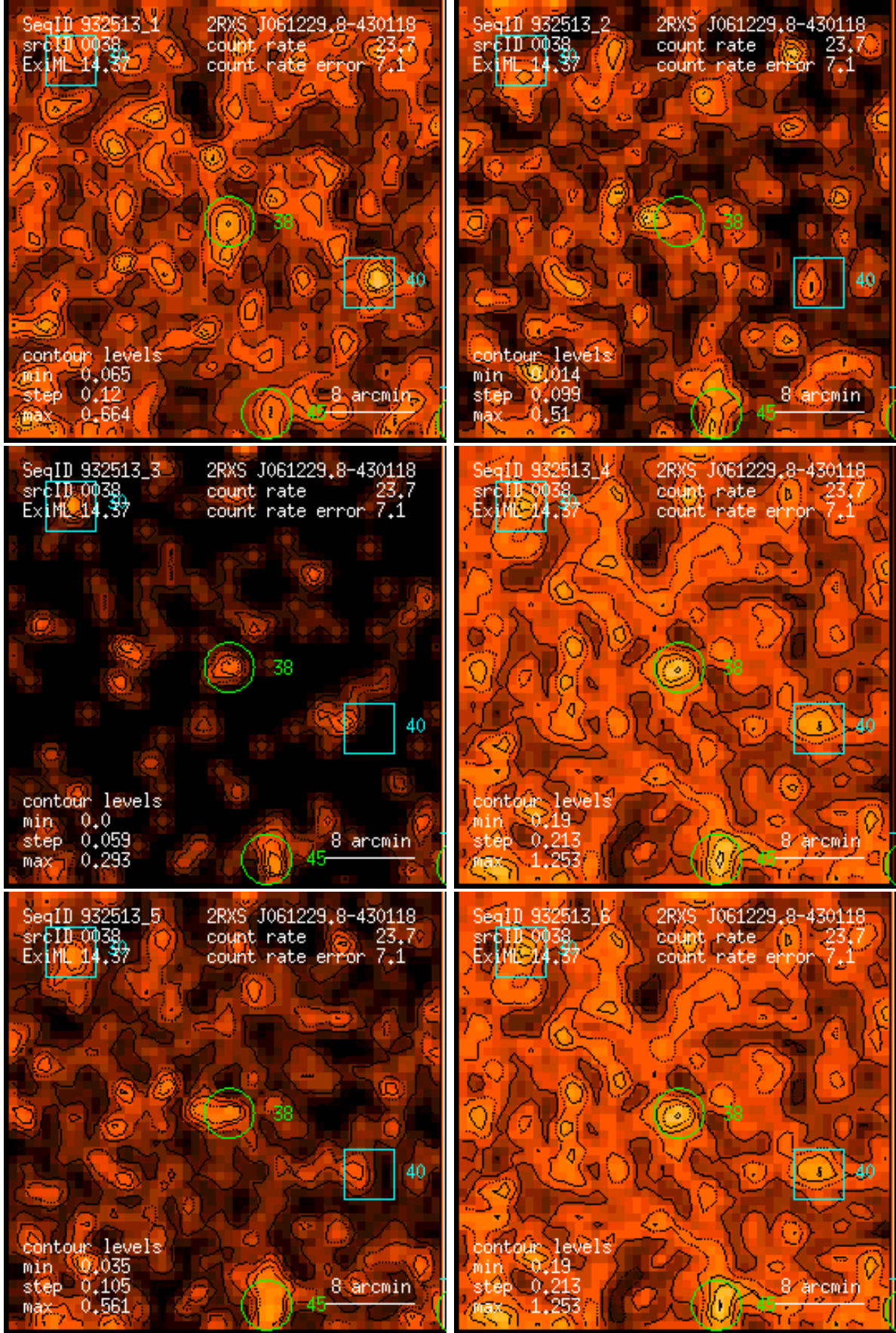
Figure 38: RASS 932513: detection 0038: band rate images, Gaussian filter: (1) PSPC channels 11 – 41, (2) 52 – 90, (3) 91 – 201, (4) 11 – 235, (5) 52 – 201, (6) 11 – 201. Broad band rates in counts/ks. Band rate contour levels in counts/ks/arcmin 2 .
