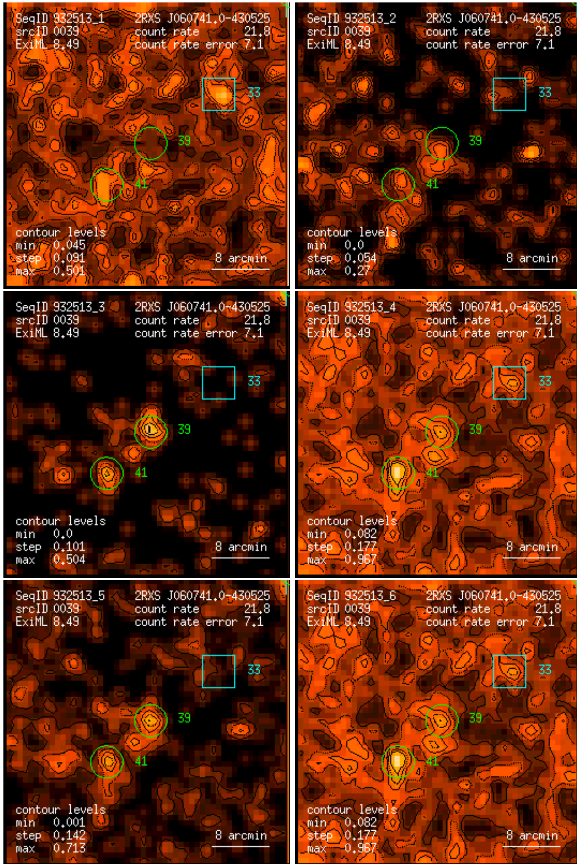
Figure 39: RASS 932513: detection 0039: band rate images, Gaussian filter: (1) PSPC channels 11 – 41, (2) 52 – 90, (3) 91 – 201, (4) 11 – 235, (5) 52 – 201, (6) 11 – 201. Broad band rates in counts/ks. Band rate contour levels in counts/ks/arcmin 2 .
