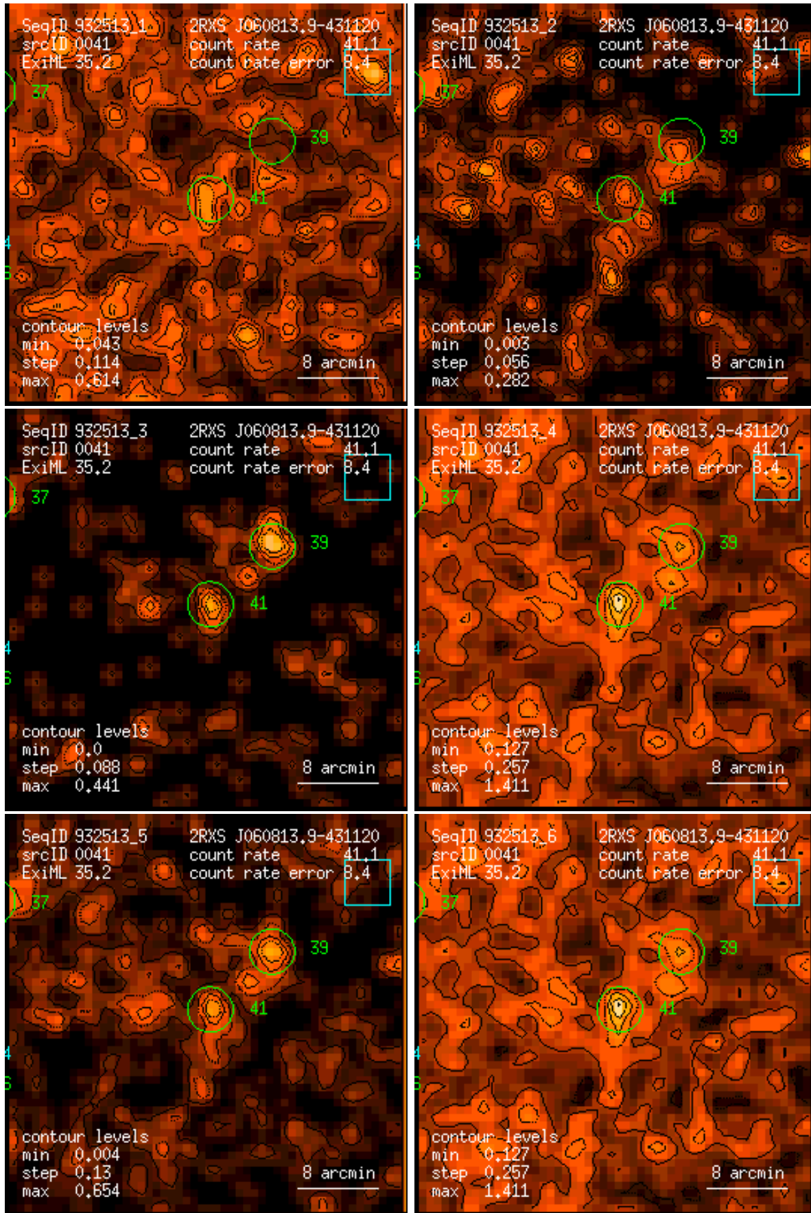
Figure 41: RASS 932513: detection 0041: band rate images, Gaussian filter: (1) PSPC channels 11 – 41, (2) 52 – 90, (3) 91 – 201, (4) 11 – 235, (5) 52 – 201, (6) 11 – 201. Broad band rates in counts/ks. Band rate contour levels in counts/ks/arcmin 2 .
