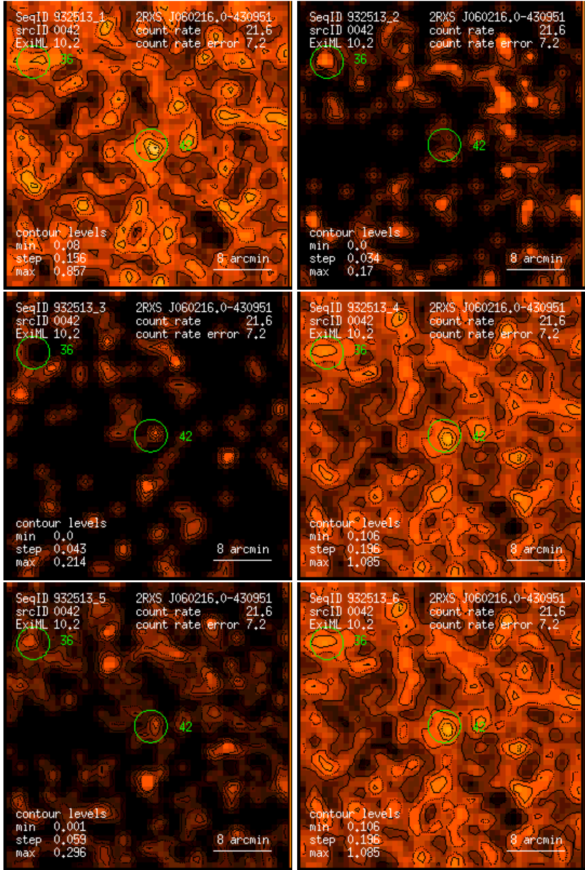
Figure 42: RASS 932513: detection 0042: band rate images, Gaussian filter: (1) PSPC channels 11 – 41, (2) 52 – 90, (3) 91 – 201, (4) 11 – 235, (5) 52 – 201, (6) 11 – 201. Broad band rates in counts/ks. Band rate contour levels in counts/ks/arcmin 2 .
