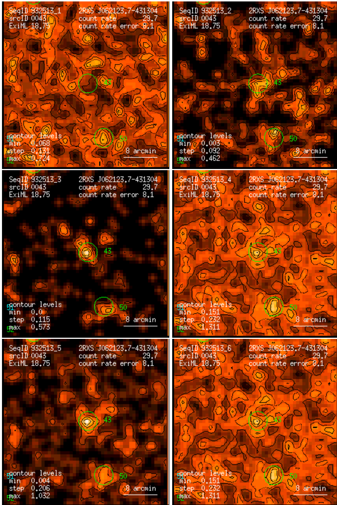
Figure 43: RASS 932513: detection 0043: band rate images, Gaussian filter: (1) PSPC channels 11 – 41, (2) 52 – 90, (3) 91 – 201, (4) 11 – 235, (5) 52 – 201, (6) 11 – 201. Broad band rates in counts/ks. Band rate contour levels in counts/ks/arcmin 2 .
