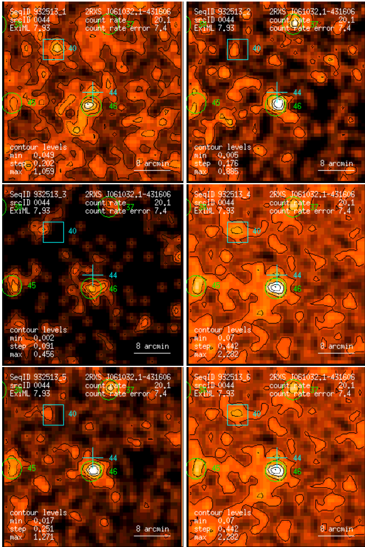
Figure 44: RASS 932513: detection 0044: band rate images, Gaussian filter: (1) PSPC channels 11 – 41, (2) 52 – 90, (3) 91 – 201, (4) 11 – 235, (5) 52 – 201, (6) 11 – 201. Broad band rates in counts/ks. Band rate contour levels in counts/ks/arcmin 2 .
