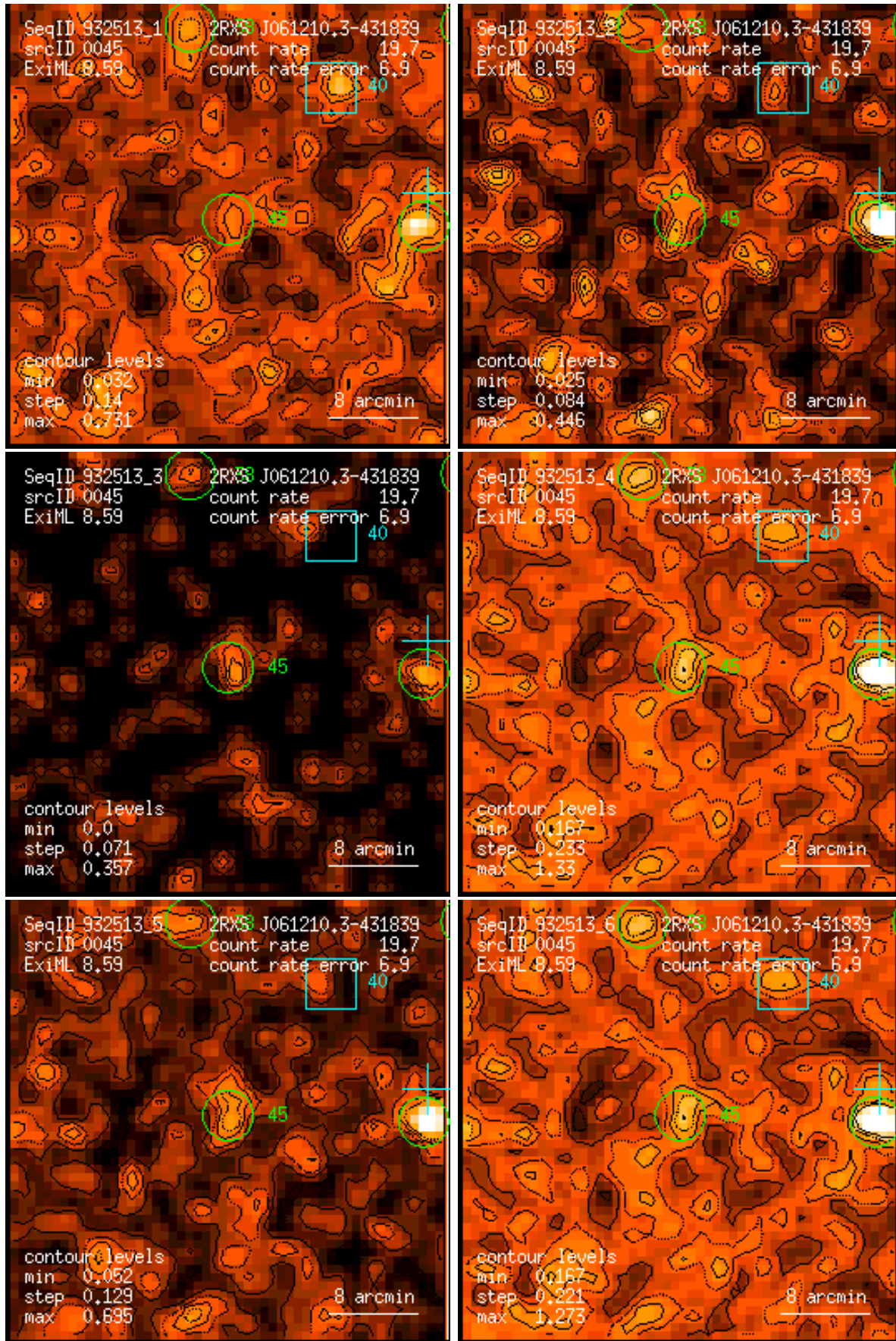
Figure 45: RASS 932513: detection 0045: band rate images, Gaussian filter: (1) PSPC channels 11 – 41, (2) 52 – 90, (3) 91 – 201, (4) 11 – 235, (5) 52 – 201, (6) 11 – 201. Broad band rates in counts/ks. Band rate contour levels in counts/ks/arcmin 2 .
