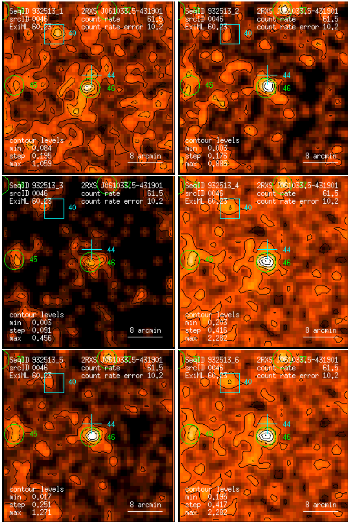
Figure 46: RASS 932513: detection 0046: band rate images, Gaussian filter: (1) PSPC channels 11 – 41, (2) 52 – 90, (3) 91 – 201, (4) 11 – 235, (5) 52 – 201, (6) 11 – 201. Broad band rates in counts/ks. Band rate contour levels in counts/ks/arcmin 2 .
