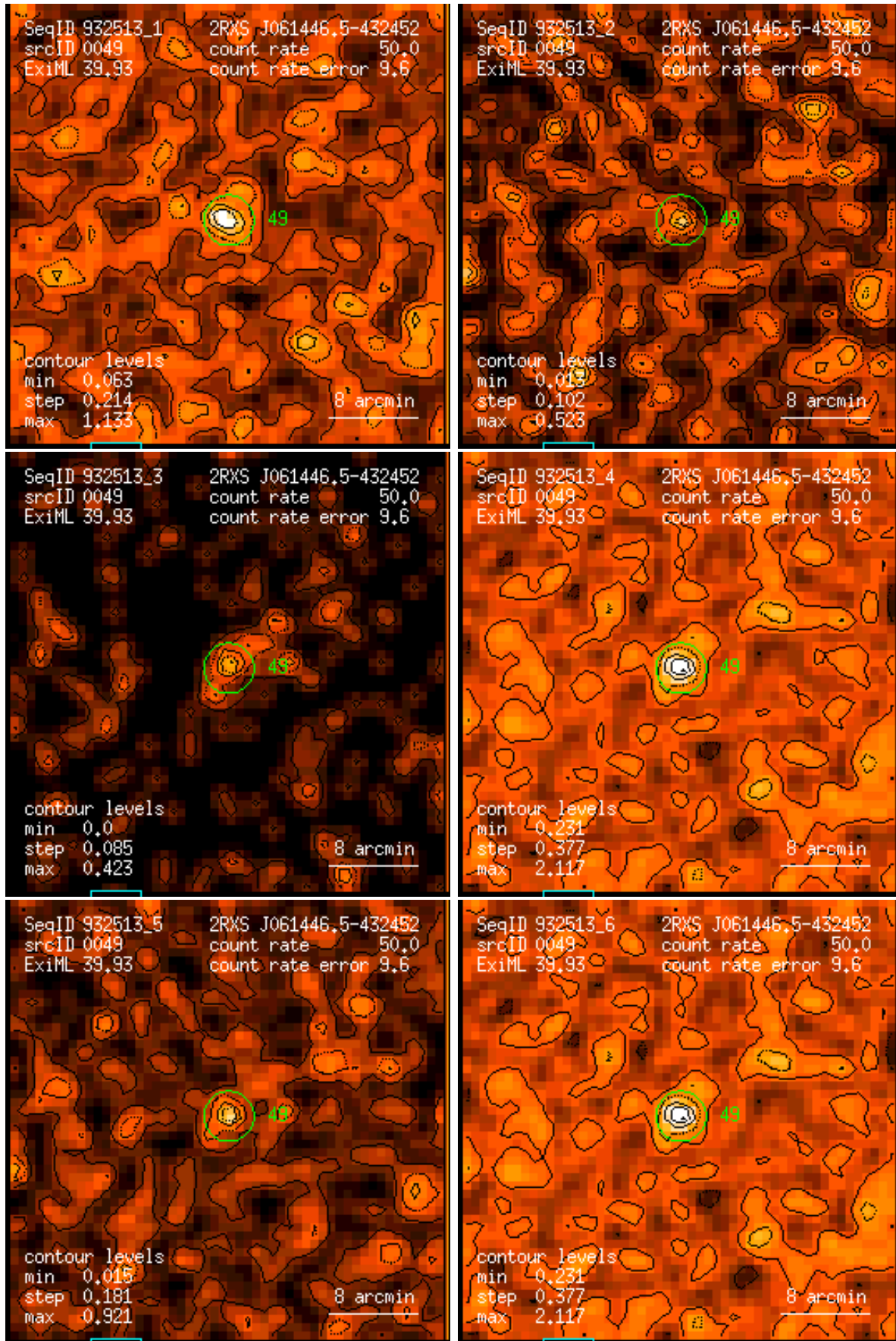
Figure 49: RASS 932513: detection 0049: band rate images, Gaussian filter: (1) PSPC channels 11 – 41, (2) 52 – 90, (3) 91 – 201, (4) 11 – 235, (5) 52 – 201, (6) 11 – 201. Broad band rates in counts/ks. Band rate contour levels in counts/ks/arcmin 2 .
