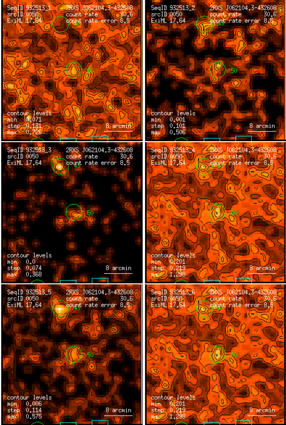
Figure 50: RASS 932513: detection 0050: band rate images, Gaussian filter: (1) PSPC channels 11 – 41, (2) 52 – 90, (3) 91 – 201, (4) 11 – 235, (5) 52 – 201, (6) 11 – 201. Broad band rates in counts/ks. Band rate contour levels in counts/ks/arcmin 2 .
