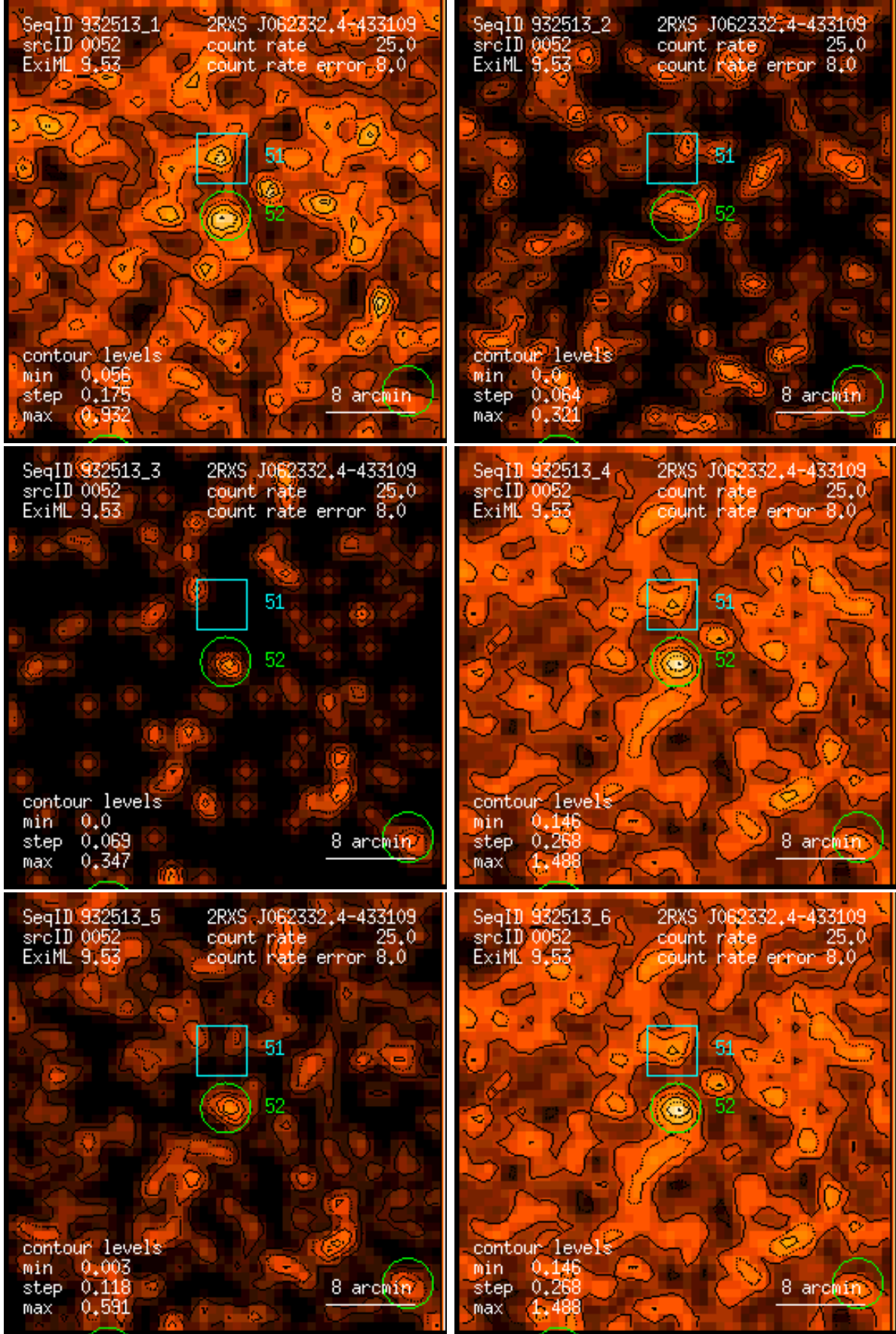
Figure 52: RASS 932513: detection 0052: band rate images, Gaussian filter: (1) PSPC channels 11 – 41, (2) 52 – 90, (3) 91 – 201, (4) 11 – 235, (5) 52 – 201, (6) 11 – 201. Broad band rates in counts/ks. Band rate contour levels in counts/ks/arcmin 2 .
