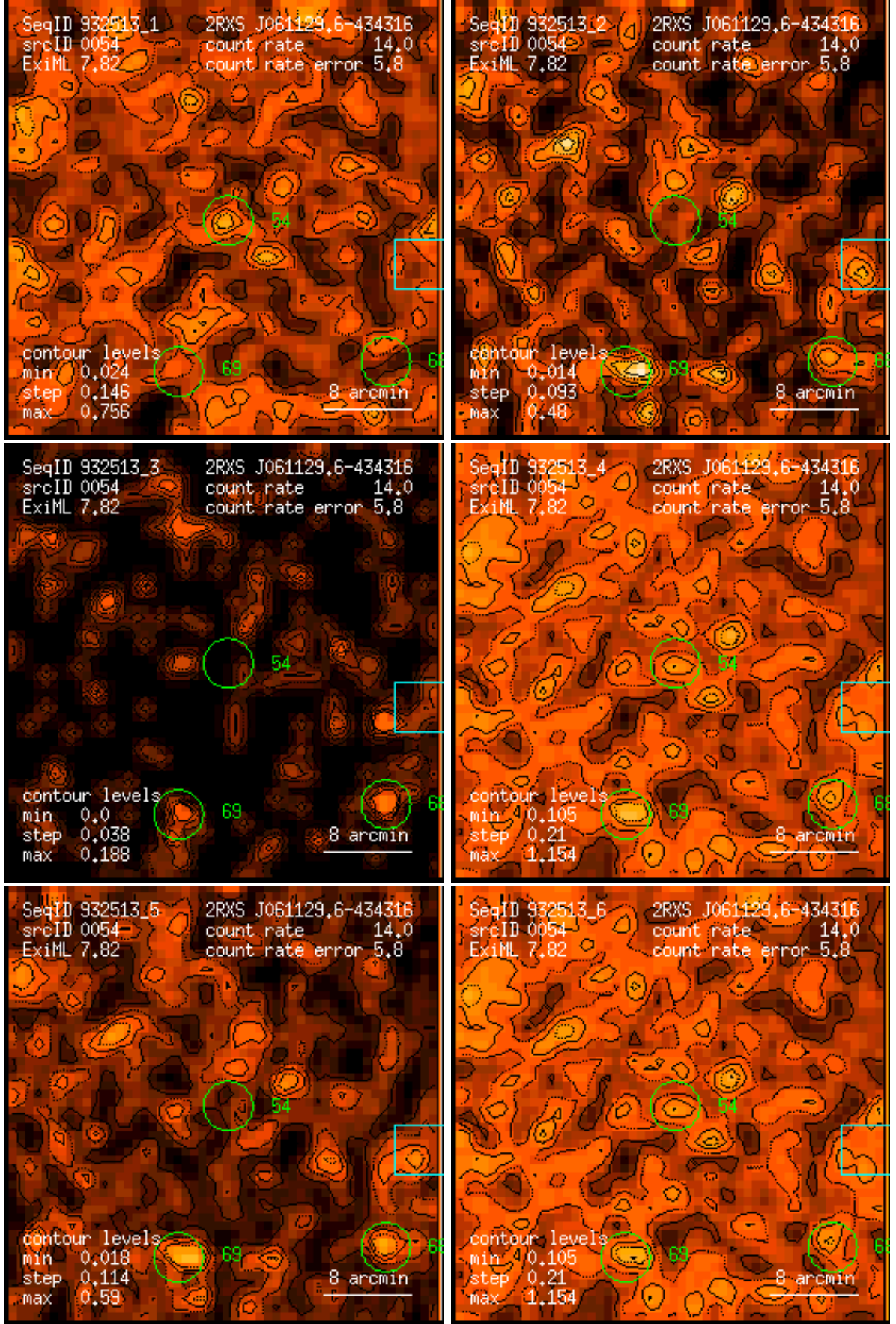
Figure 54: RASS 932513: detection 0054: band rate images, Gaussian filter: (1) PSPC channels 11 – 41, (2) 52 – 90, (3) 91 – 201, (4) 11 – 235, (5) 52 – 201, (6) 11 – 201. Broad band rates in counts/ks. Band rate contour levels in counts/ks/arcmin 2 .
