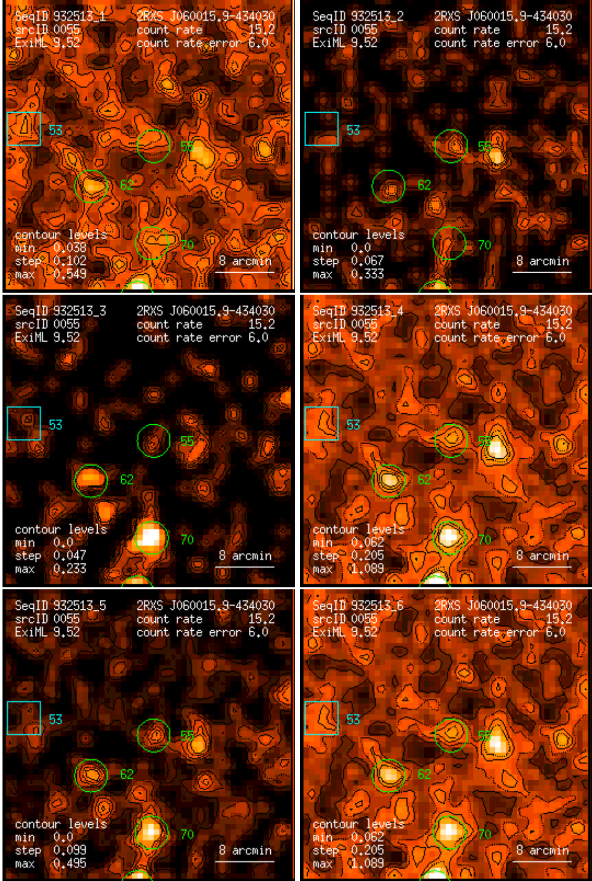
Figure 55: RASS 932513: detection 0055: band rate images, Gaussian filter: (1) PSPC channels 11 – 41, (2) 52 – 90, (3) 91 – 201, (4) 11 – 235, (5) 52 – 201, (6) 11 – 201. Broad band rates in counts/ks. Band rate contour levels in counts/ks/arcmin 2 .
