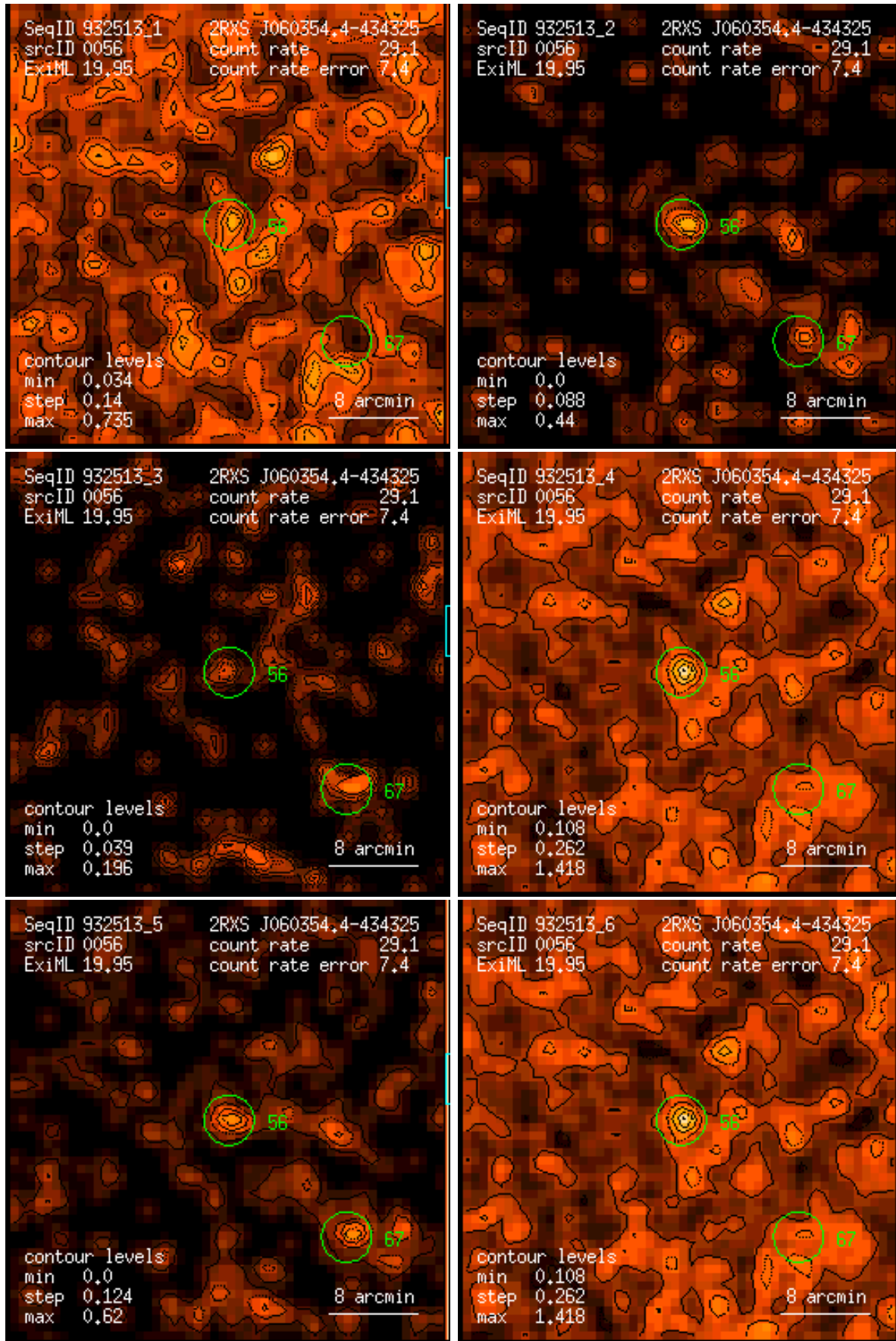
Figure 56: RASS 932513: detection 0056: band rate images, Gaussian filter: (1) PSPC channels 11 – 41, (2) 52 – 90, (3) 91 – 201, (4) 11 – 235, (5) 52 – 201, (6) 11 – 201. Broad band rates in counts/ks. Band rate contour levels in counts/ks/arcmin 2 .
