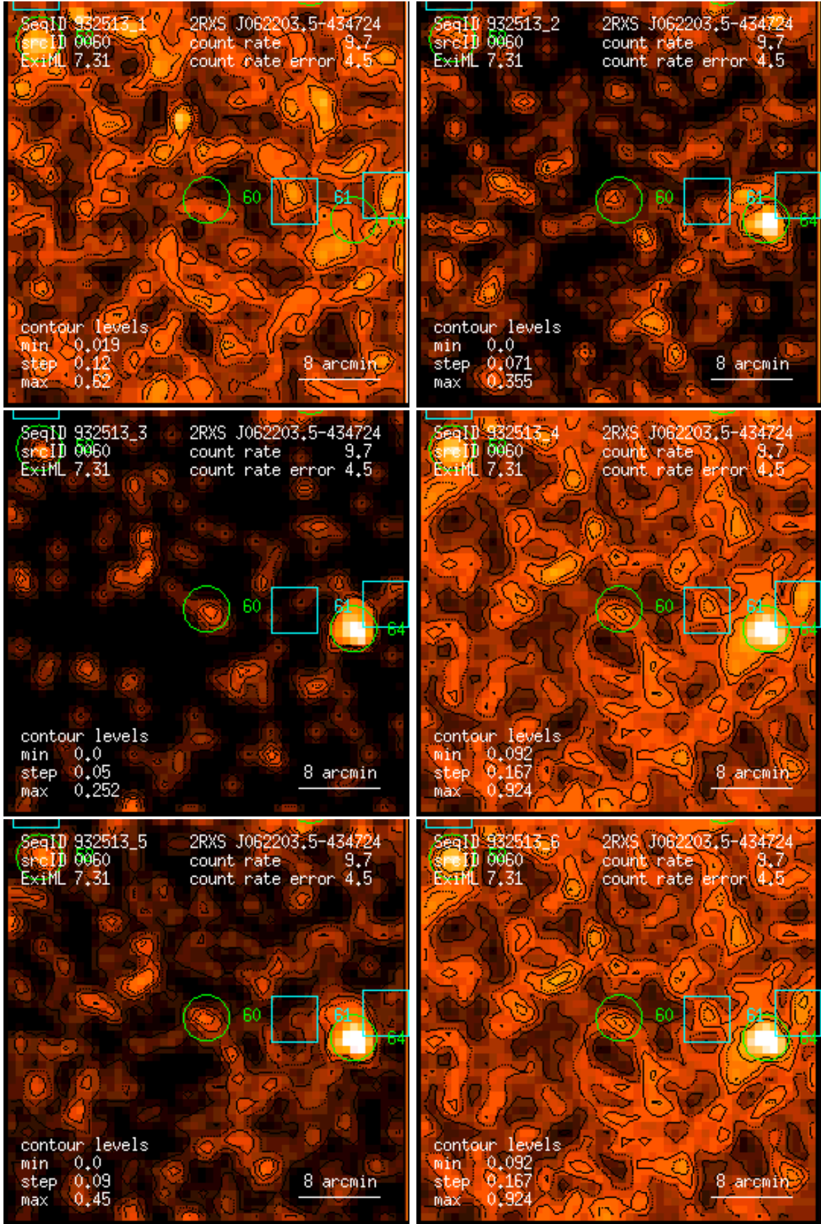
Figure 60: RASS 932513: detection 0060: band rate images, Gaussian filter: (1) PSPC channels 11 – 41, (2) 52 – 90, (3) 91 – 201, (4) 11 – 235, (5) 52 – 201, (6) 11 – 201. Broad band rates in counts/ks. Band rate contour levels in counts/ks/arcmin 2 .
