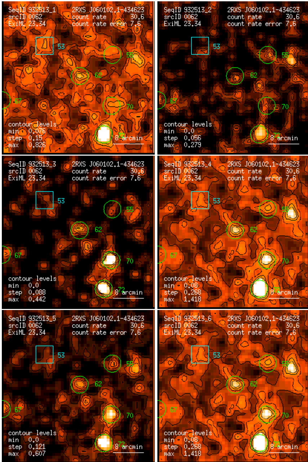
Figure 62: RASS 932513: detection 0062: band rate images, Gaussian filter: (1) PSPC channels 11 – 41, (2) 52 – 90, (3) 91 – 201, (4) 11 – 235, (5) 52 – 201, (6) 11 – 201. Broad band rates in counts/ks. Band rate contour levels in counts/ks/arcmin 2 .
