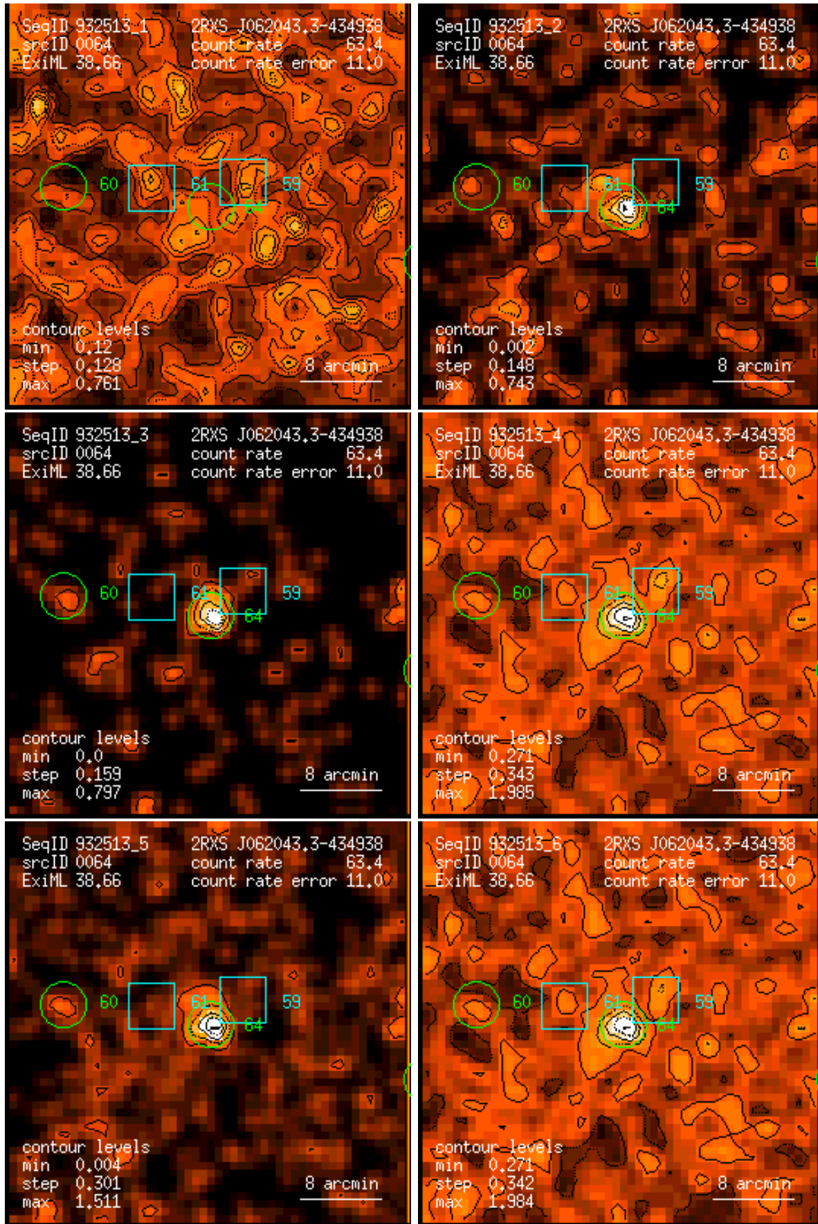
Figure 64: RASS 932513: detection 0064: band rate images, Gaussian filter: (1) PSPC channels 11 – 41, (2) 52 – 90, (3) 91 – 201, (4) 11 – 235, (5) 52 – 201, (6) 11 – 201. Broad band rates in counts/ks. Band rate contour levels in counts/ks/arcmin 2 .
