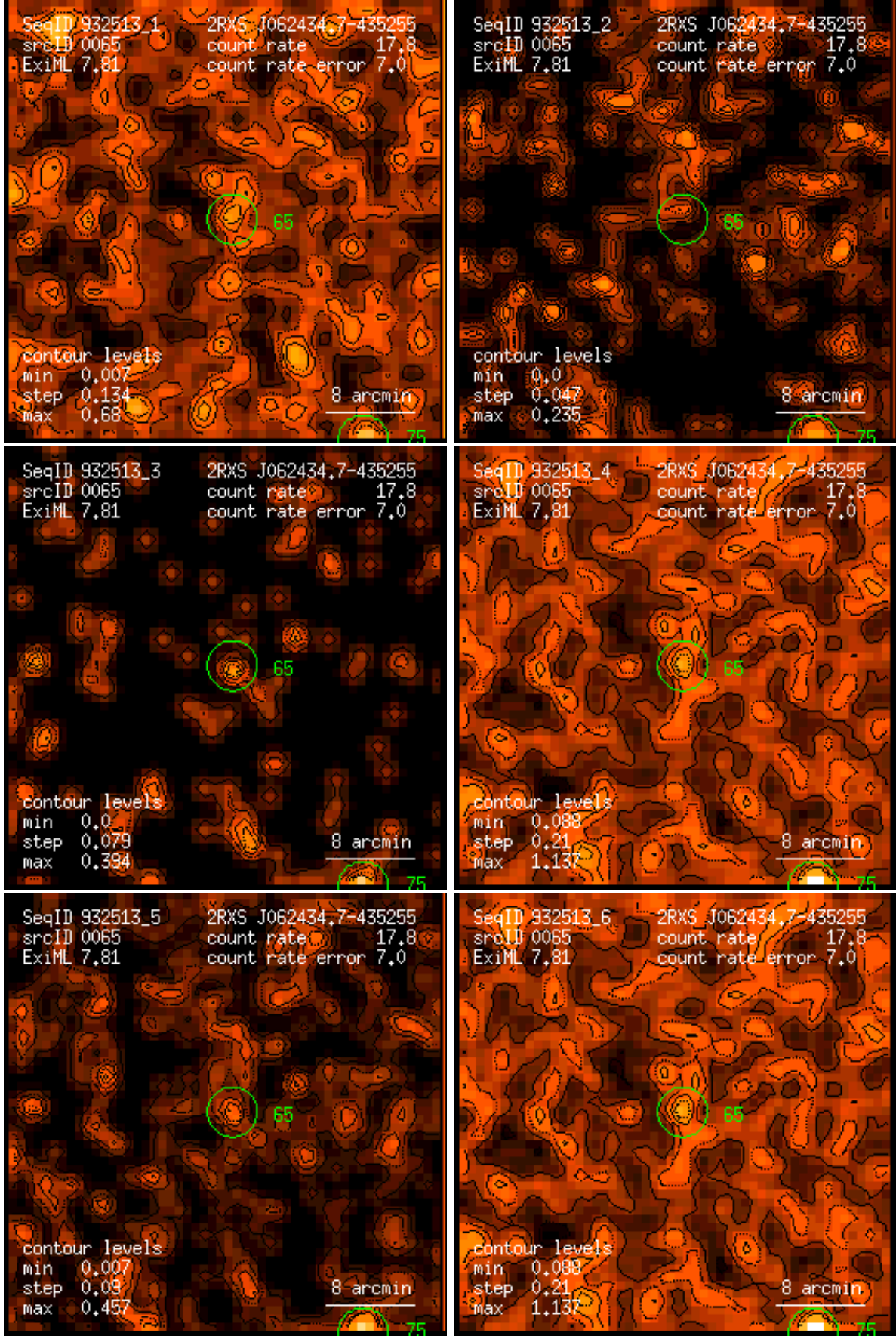
Figure 65: RASS 932513: detection 0065: band rate images, Gaussian filter: (1) PSPC channels 11 – 41, (2) 52 – 90, (3) 91 – 201, (4) 11 – 235, (5) 52 – 201, (6) 11 – 201. Broad band rates in counts/ks. Band rate contour levels in counts/ks/arcmin 2 .
