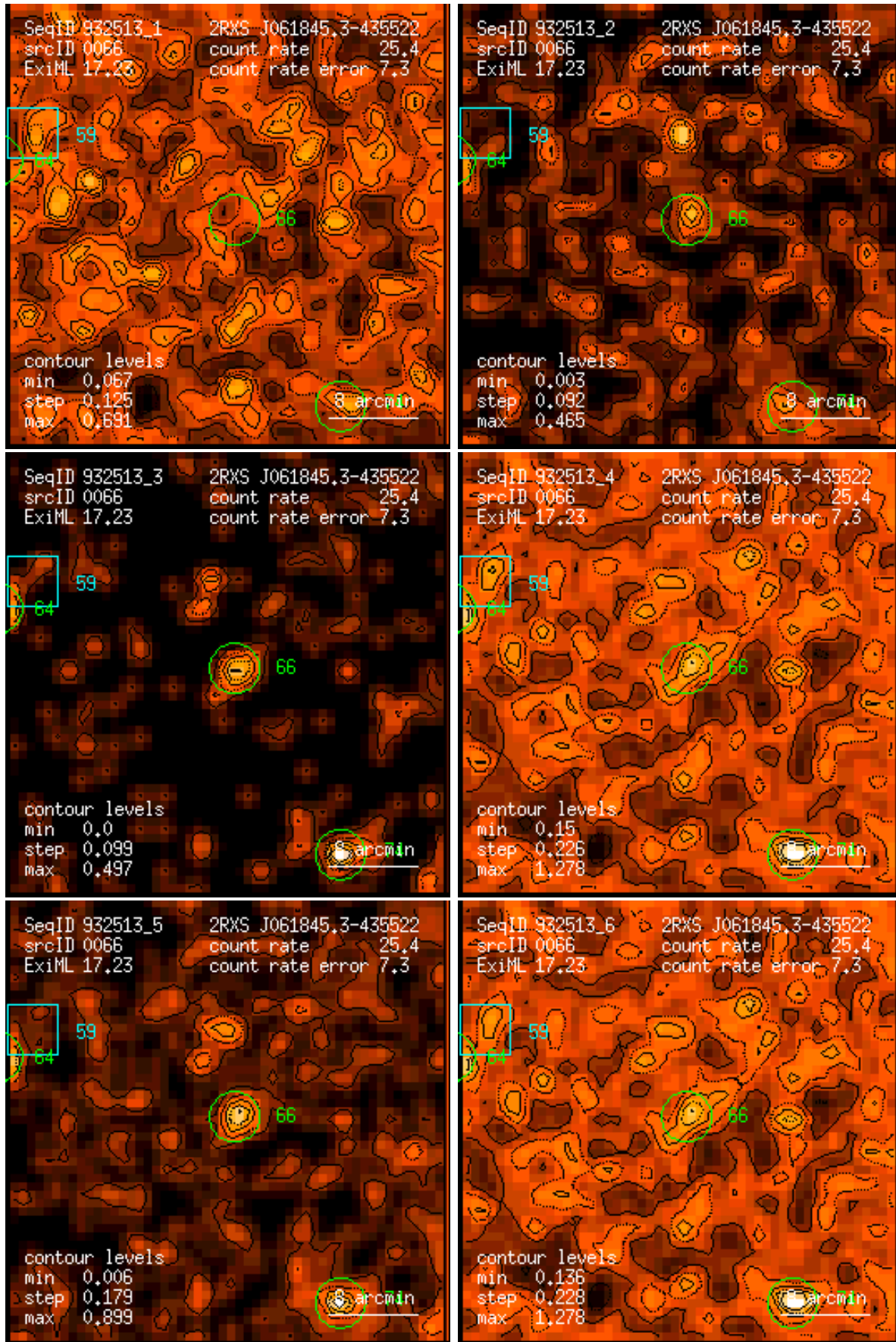
Figure 66: RASS 932513: detection 0066: band rate images, Gaussian filter: (1) PSPC channels 11 – 41, (2) 52 – 90, (3) 91 – 201, (4) 11 – 235, (5) 52 – 201, (6) 11 – 201. Broad band rates in counts/ks. Band rate contour levels in counts/ks/arcmin 2 .
